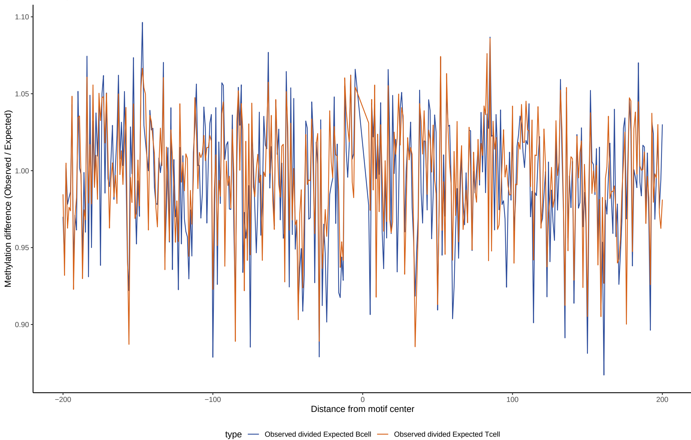
TF footprint difference for GBX2
