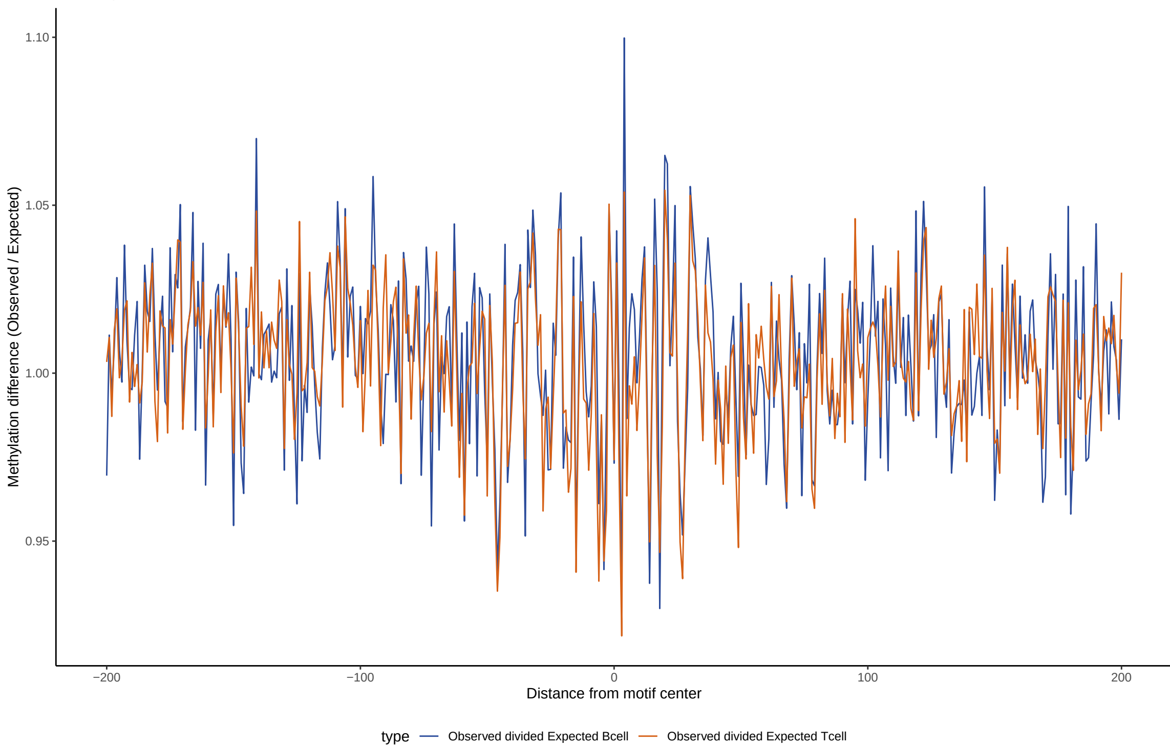
TF footprint difference for GLIS3
