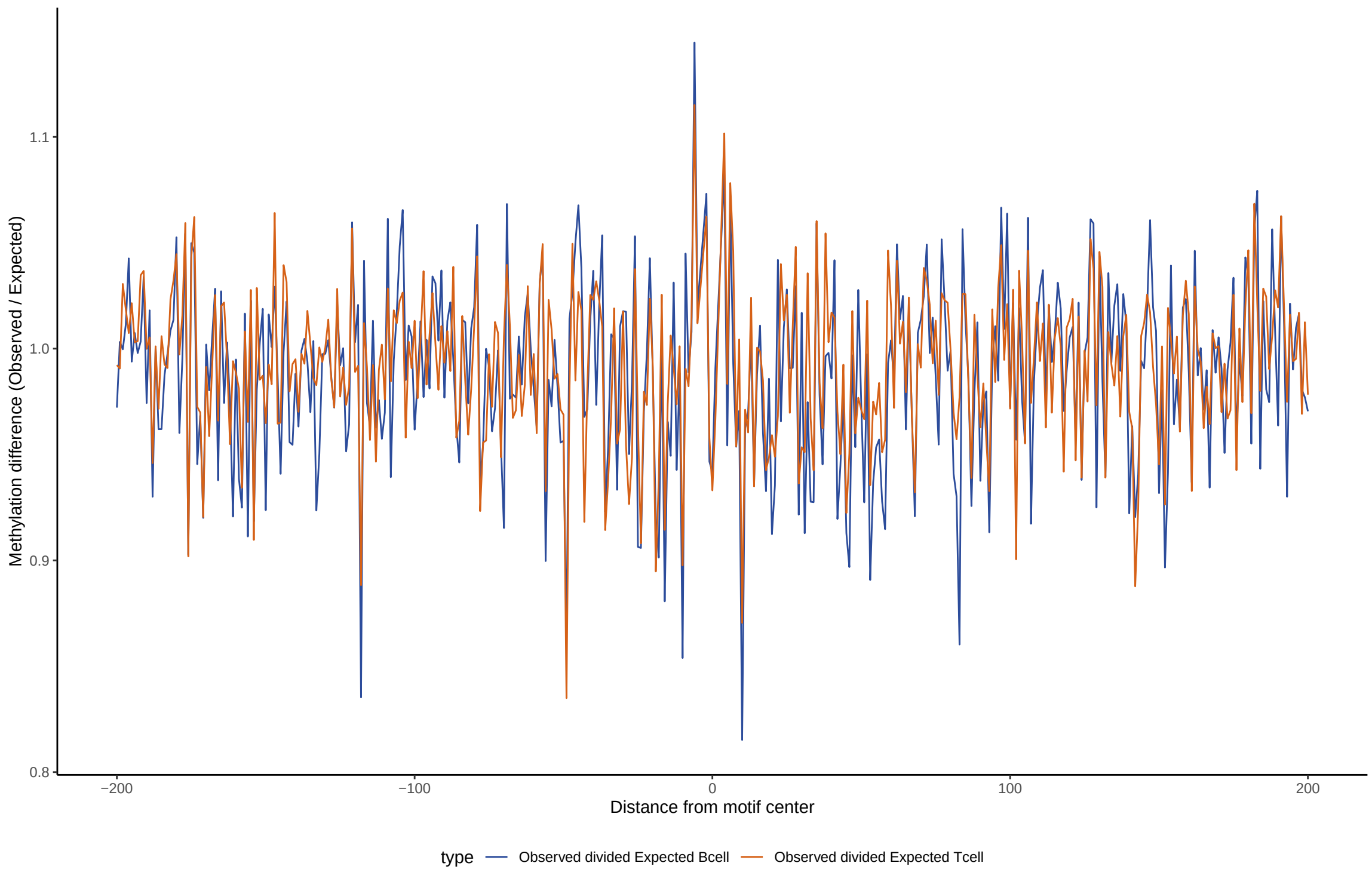
TF footprint difference for GRHL1
