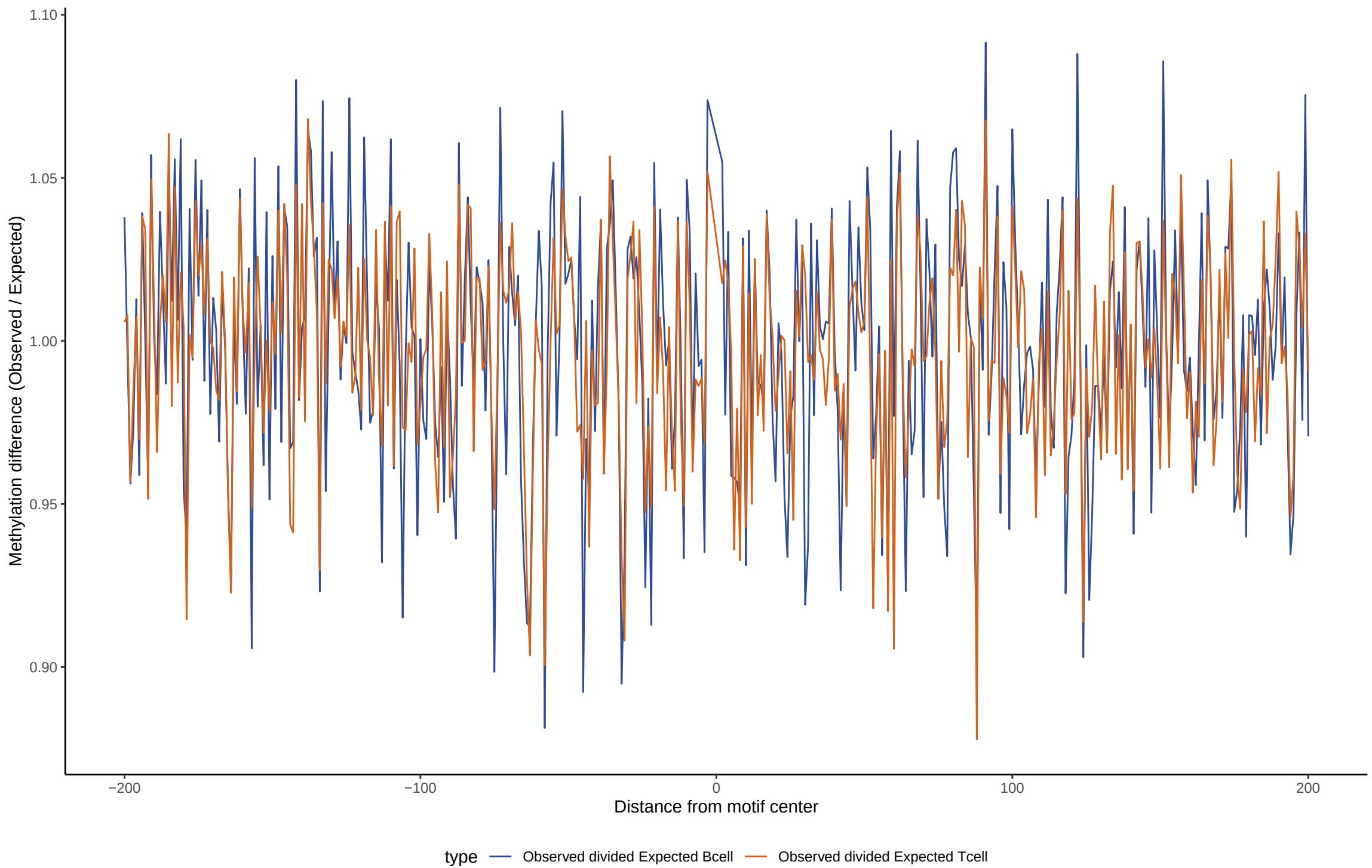
TF footprint difference for GSC
