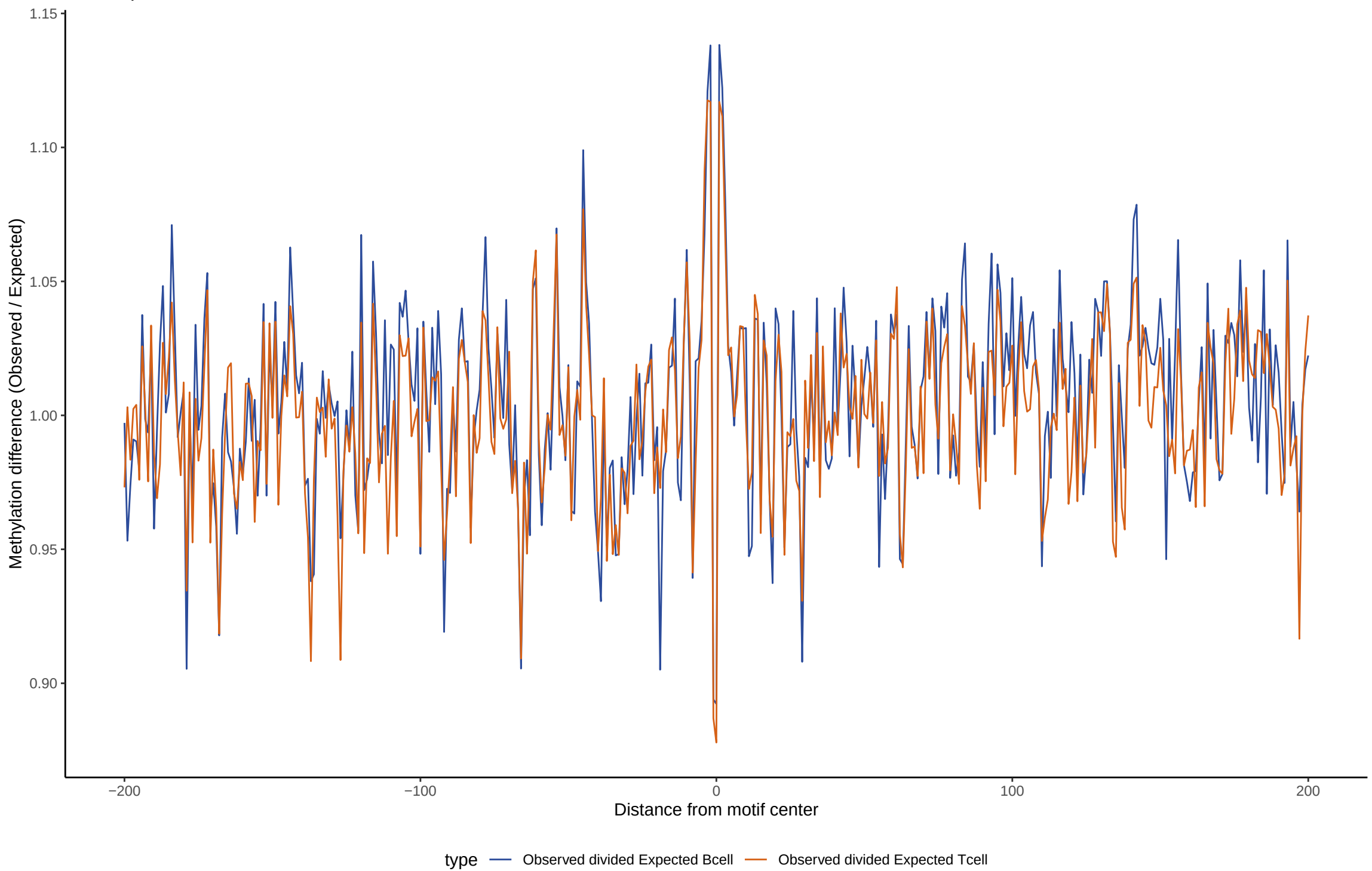
TF footprint difference for HEY1
