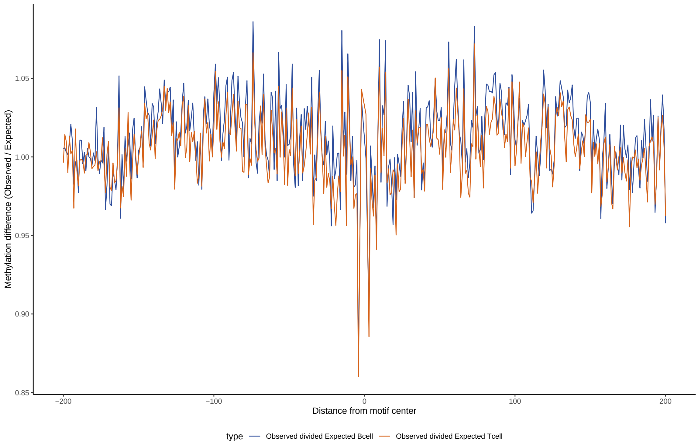
TF footprint difference for HIC2
