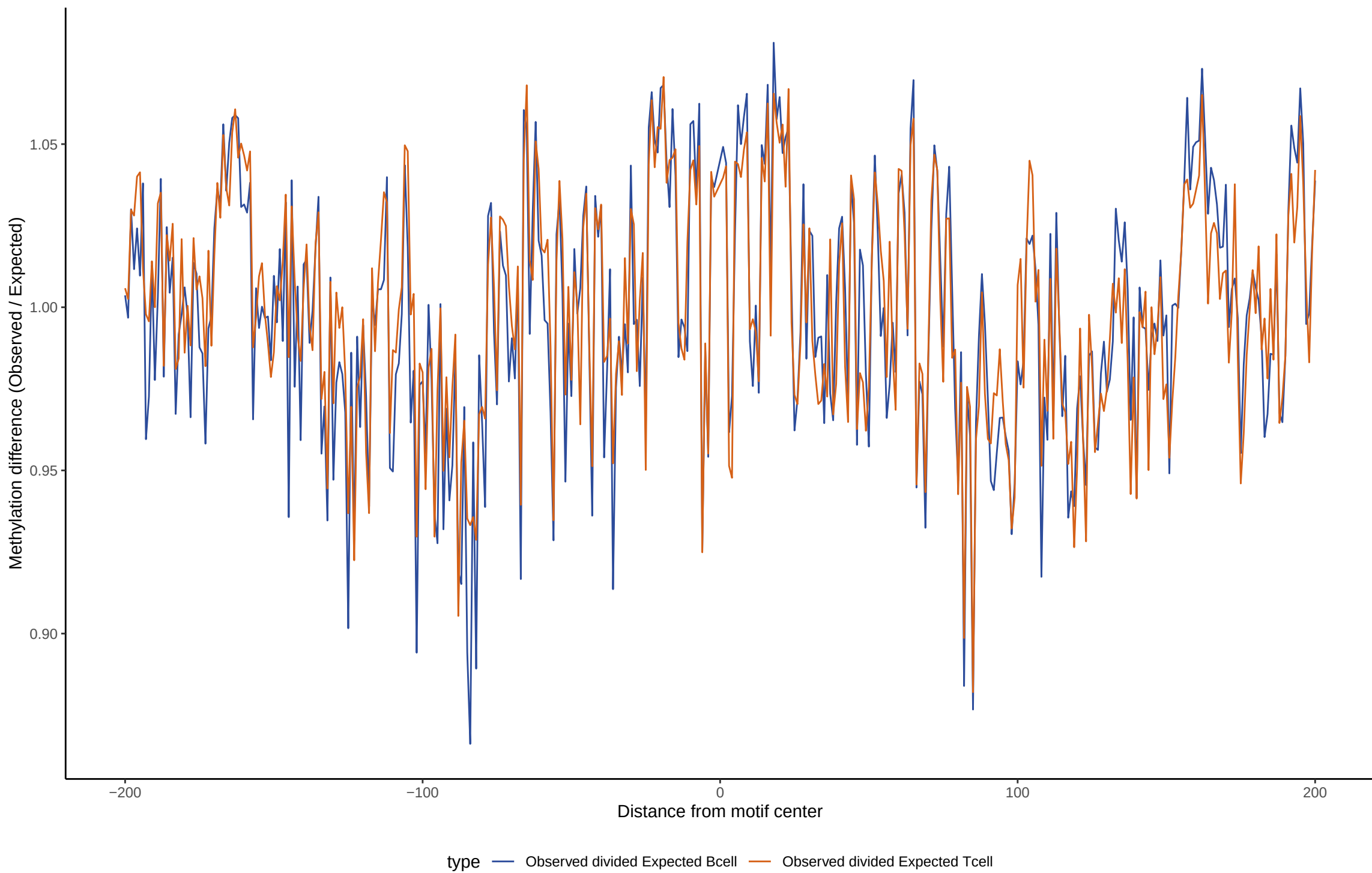
TF footprint difference for HINFP
