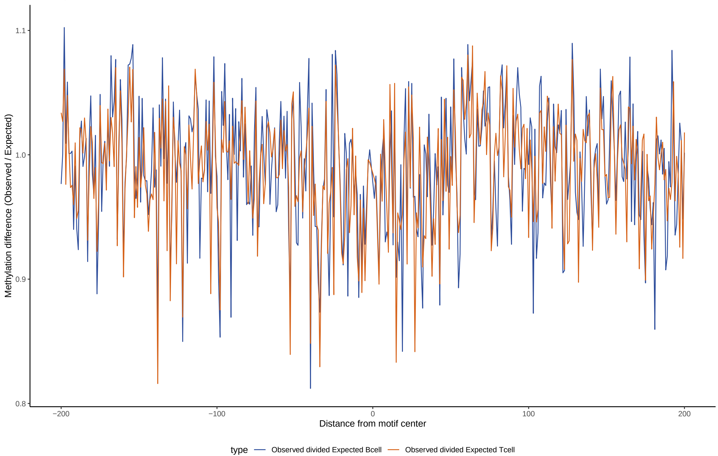
TF footprint difference for HOXD11
