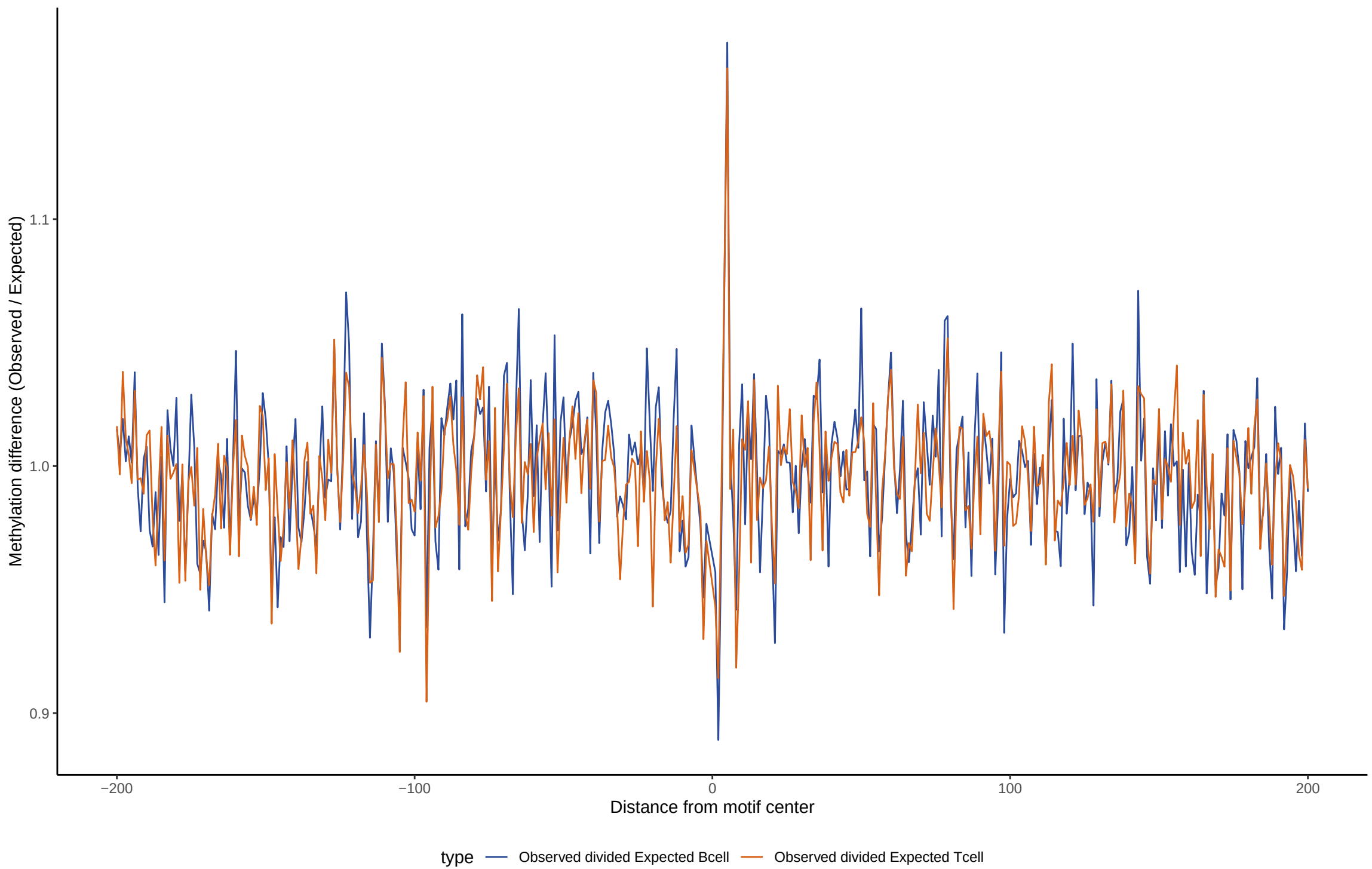
TF footprint difference for HSF1
