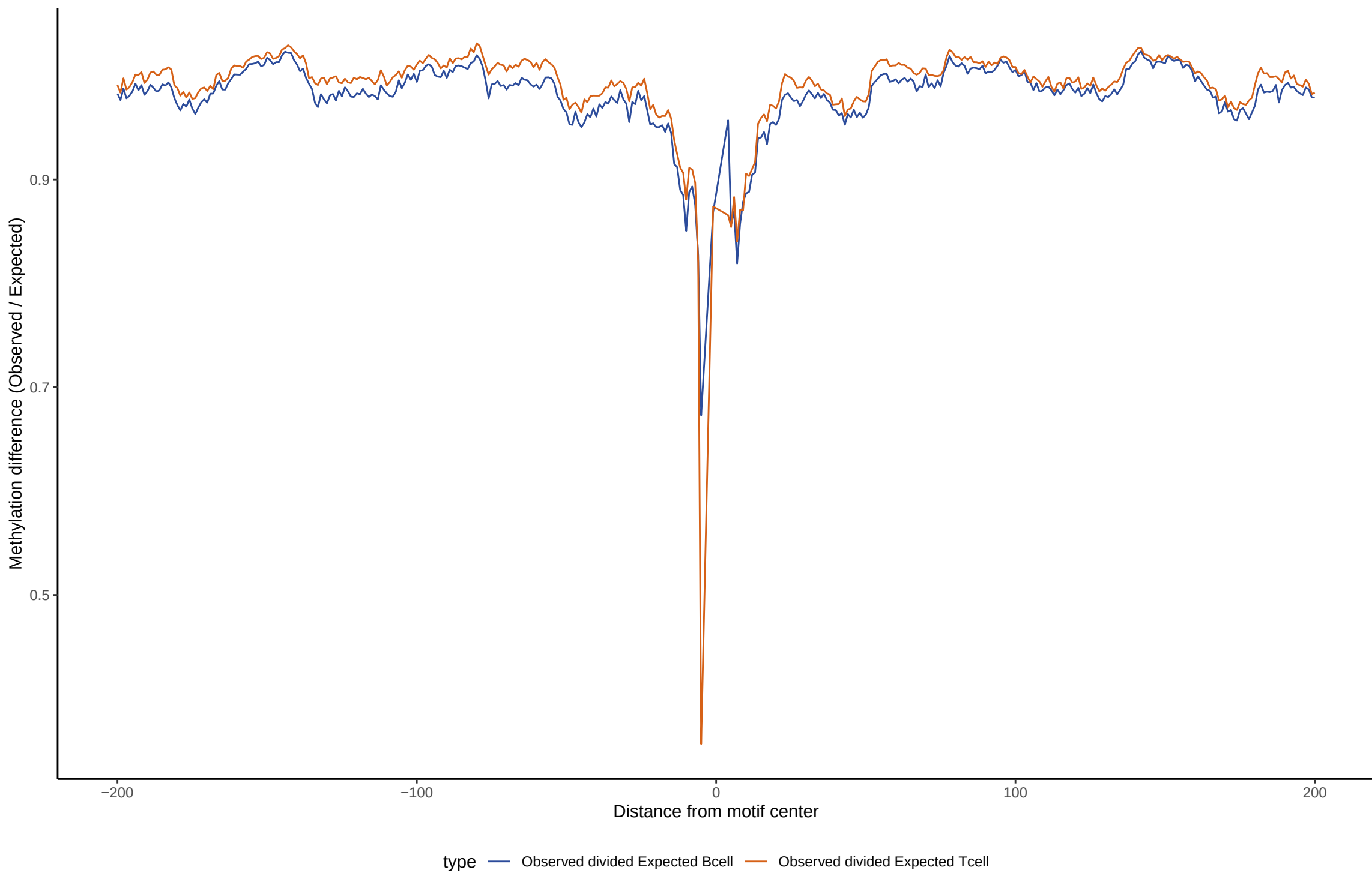
TF footprint difference for IRF1
