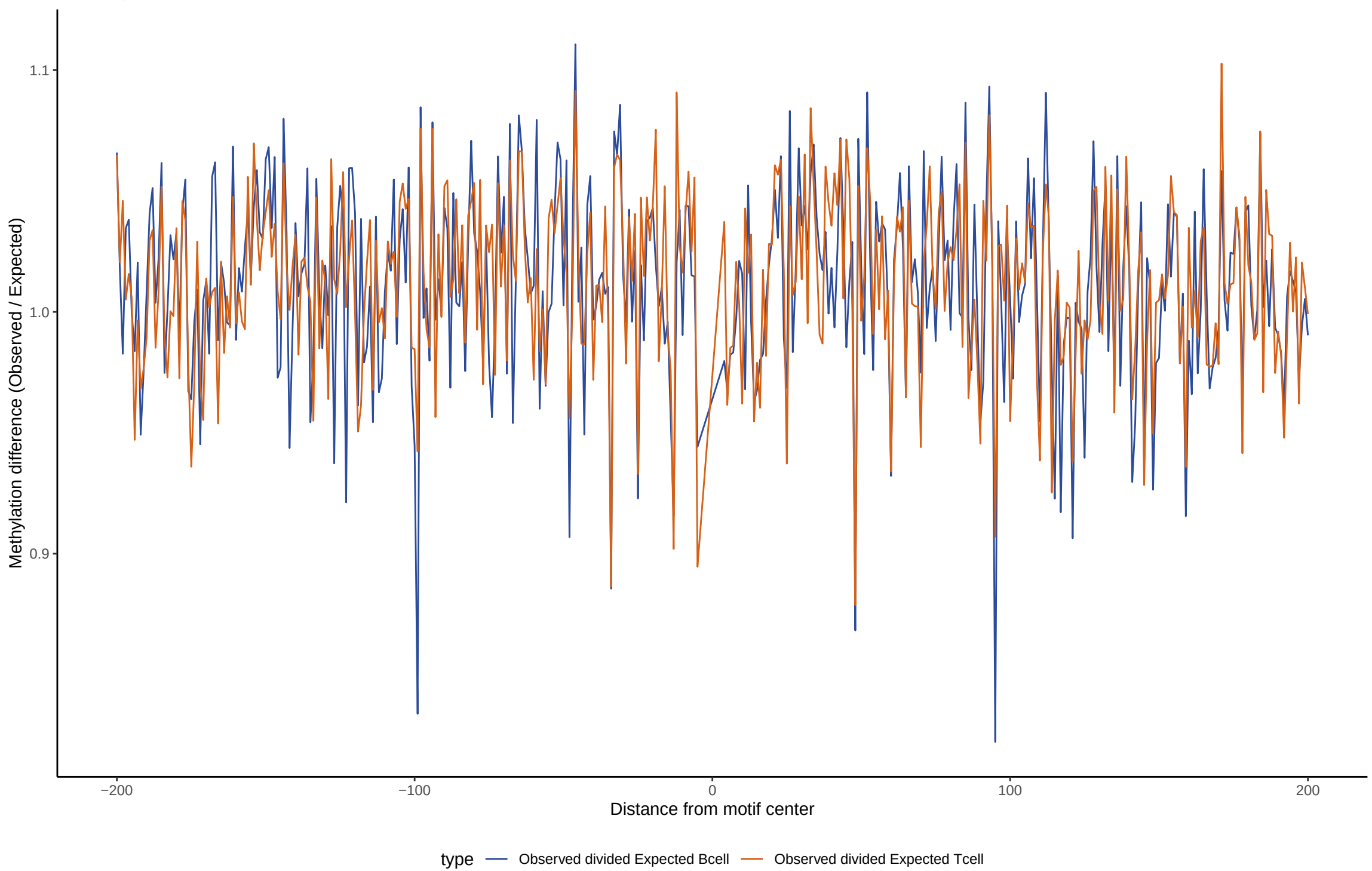
TF footprint difference for ISX
