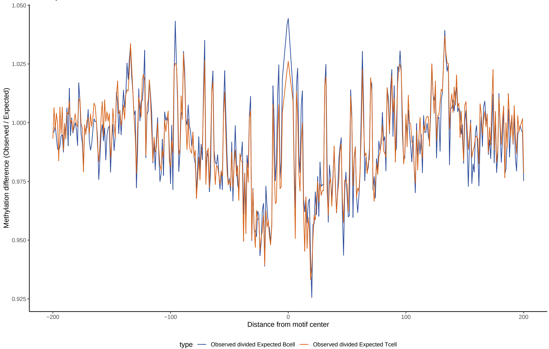
TF footprint difference for KLF5
