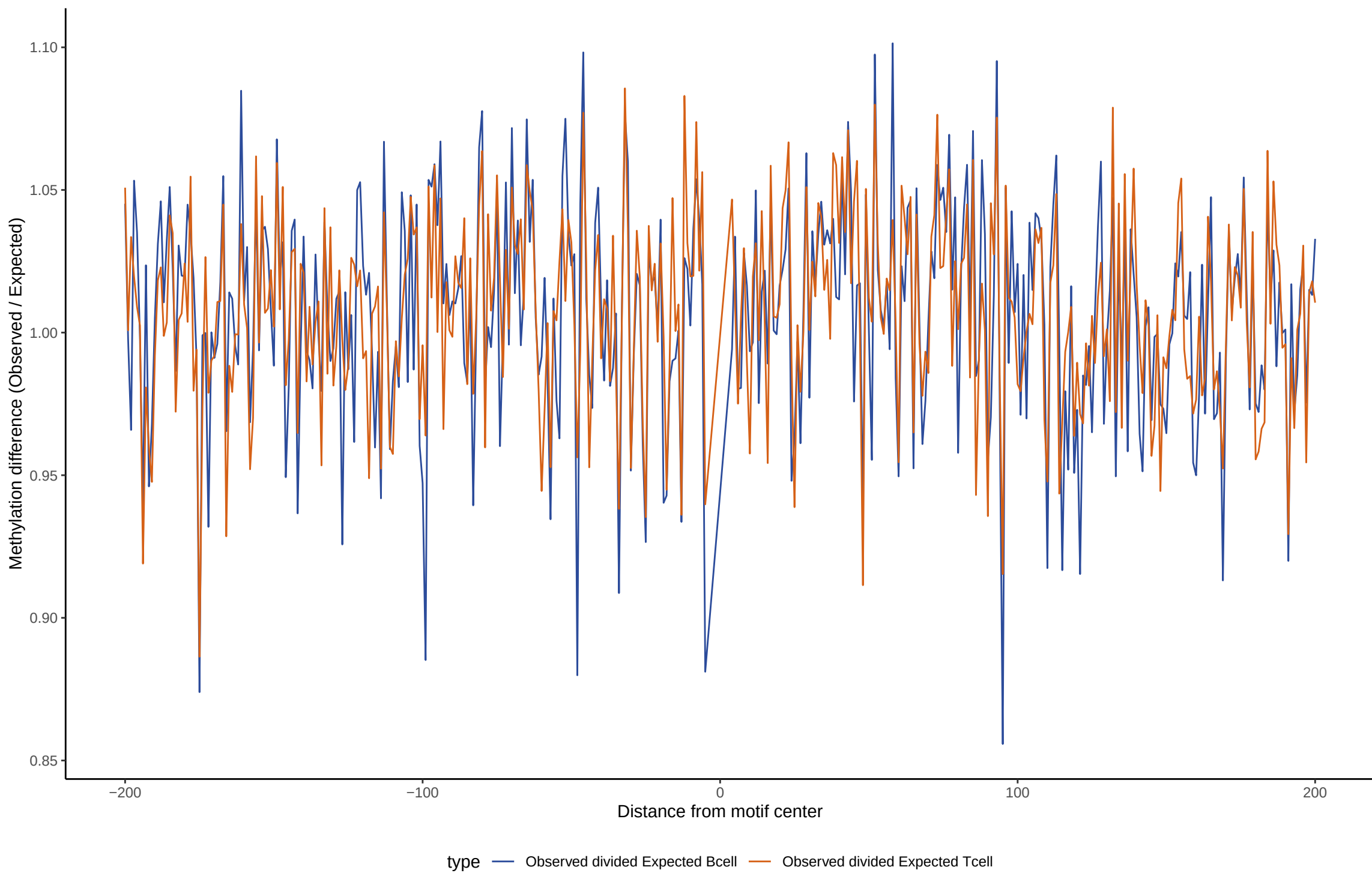
TF footprint difference for LBX1
