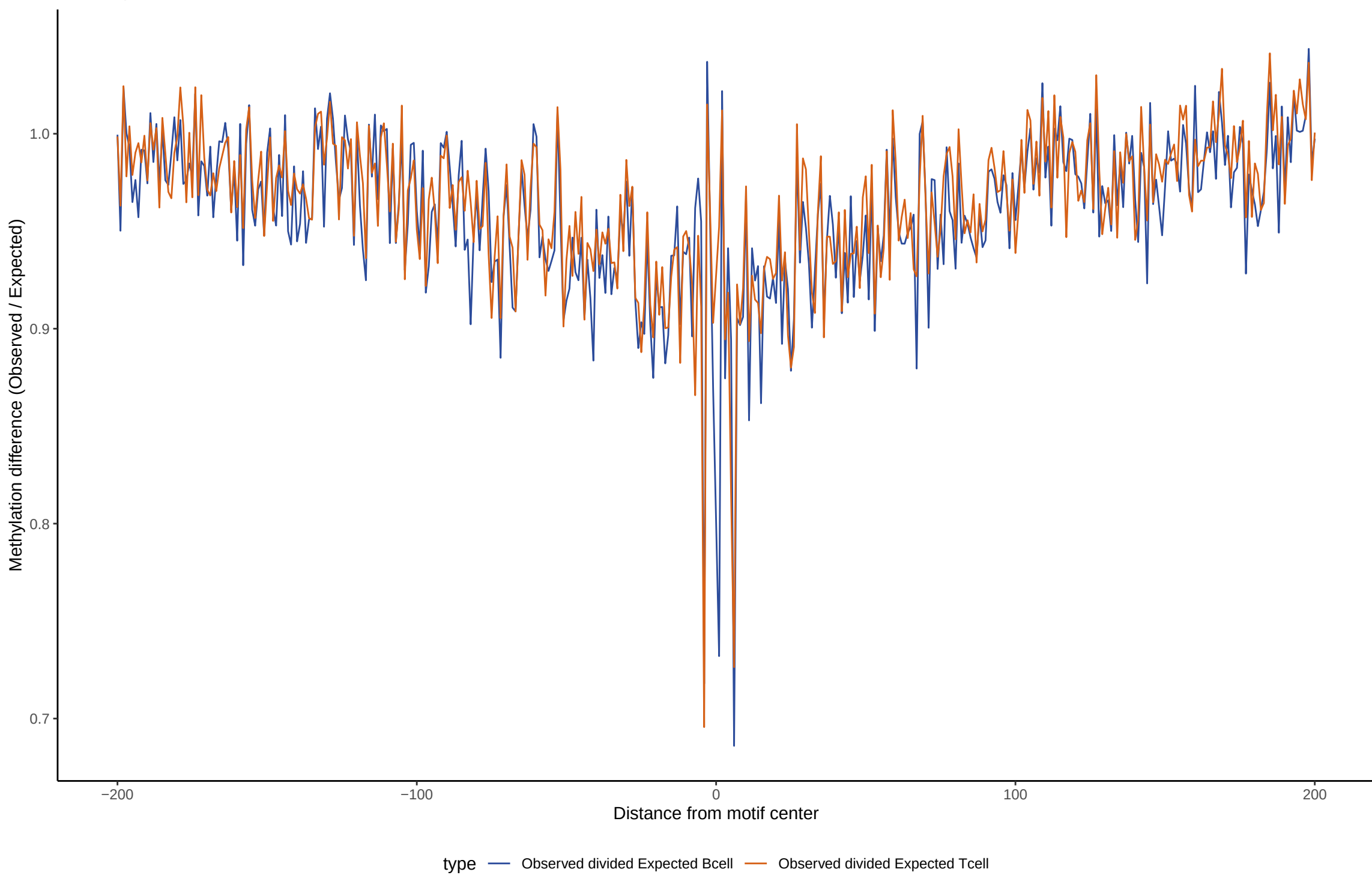
TF footprint difference for MAF::NFE2
