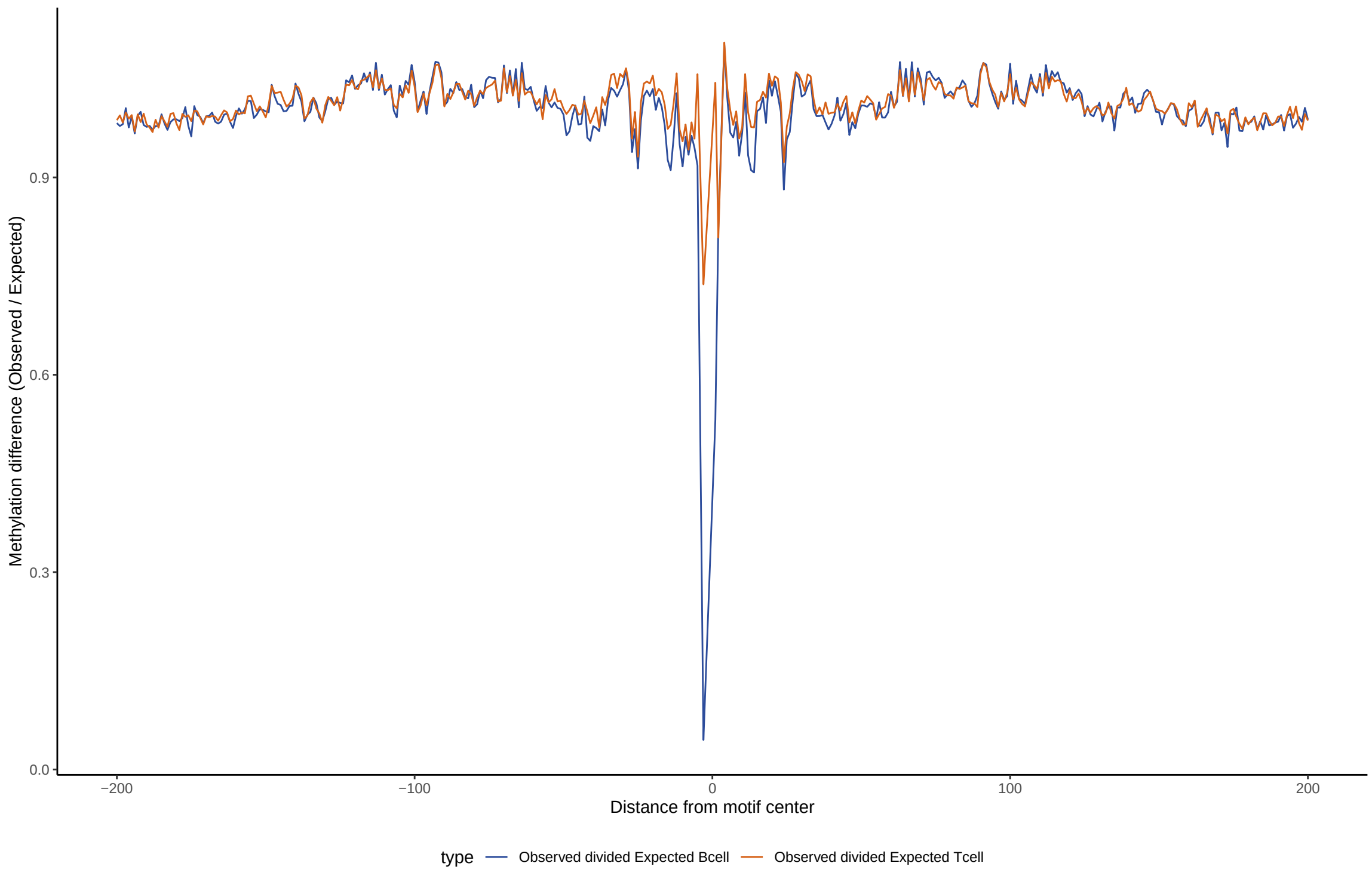
TF footprint difference for MEF2C
