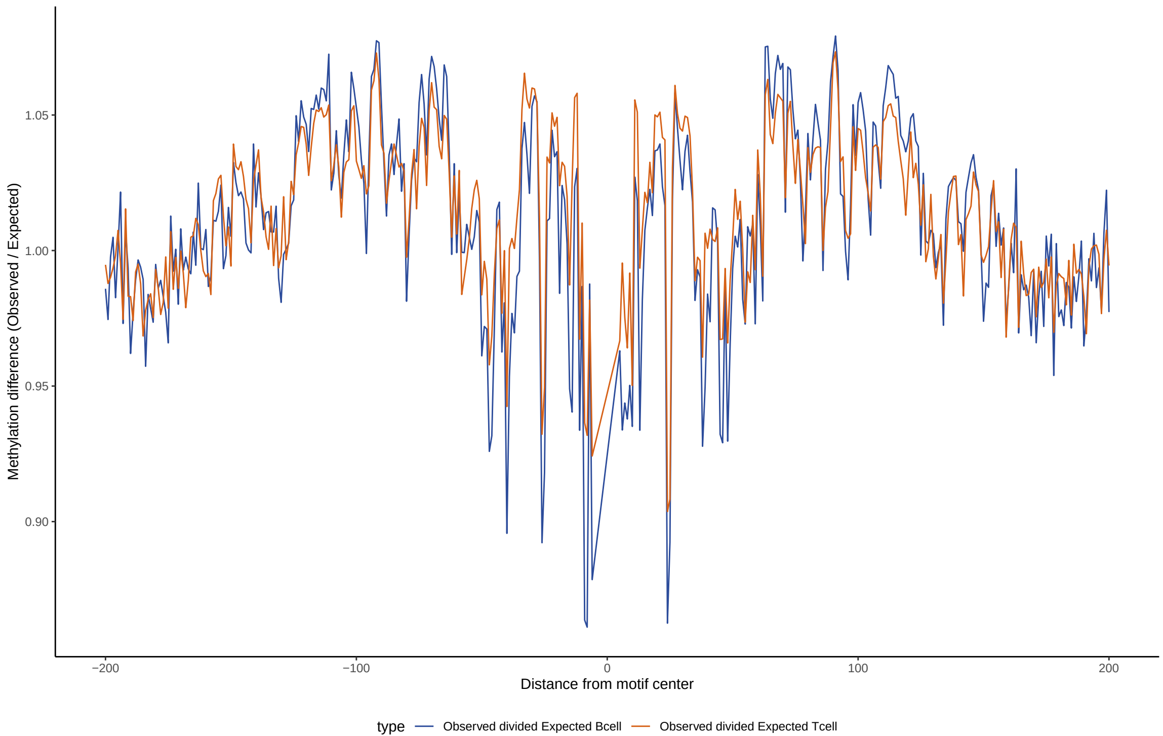
TF footprint difference for MEF2D
