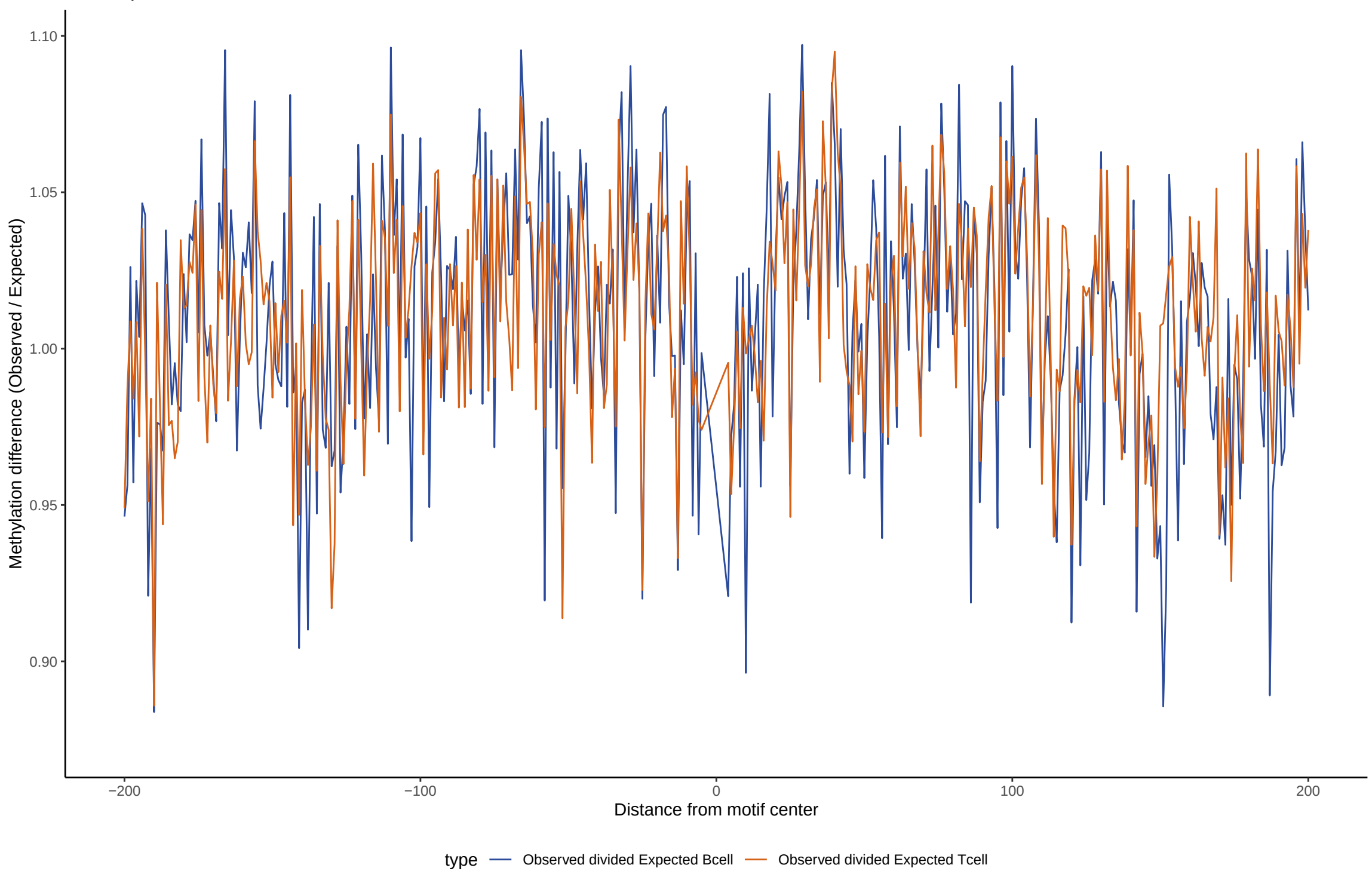
TF footprint difference for MIXL1
