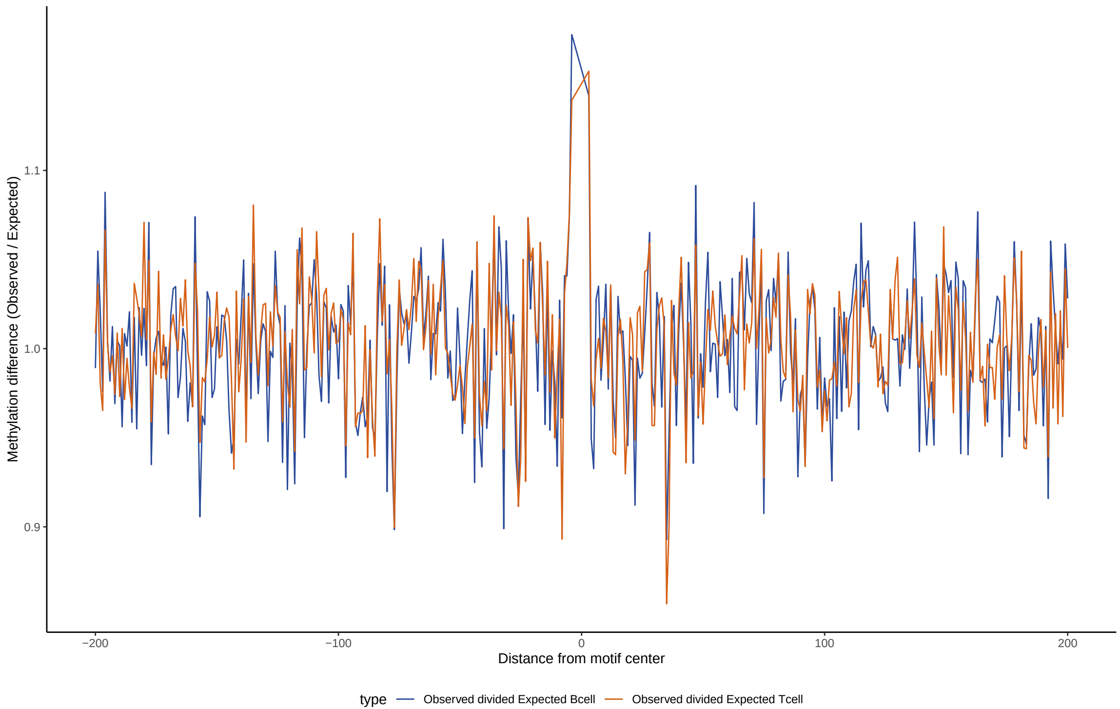
TF footprint difference for MSX1
