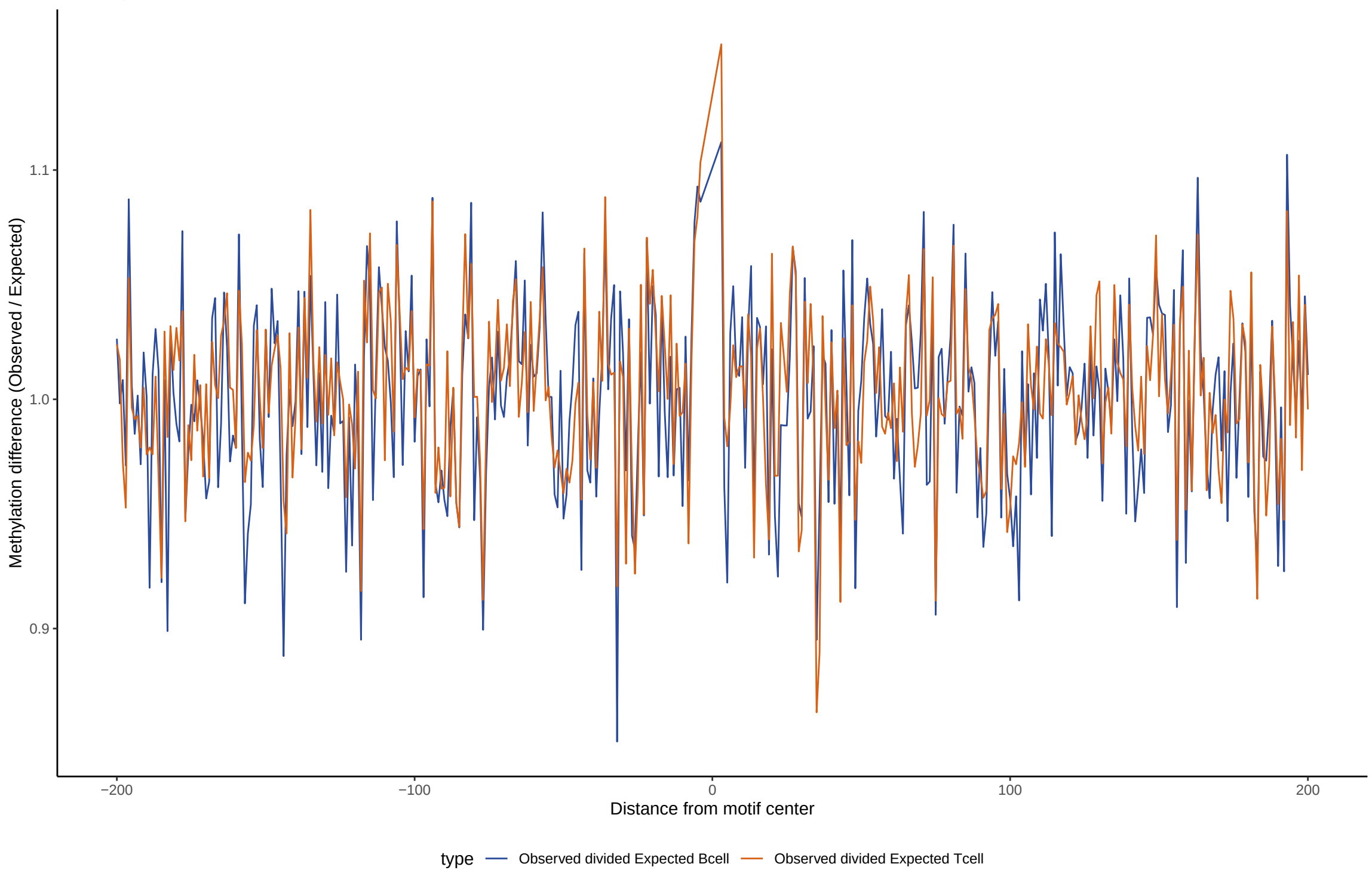
TF footprint difference for MSX2
