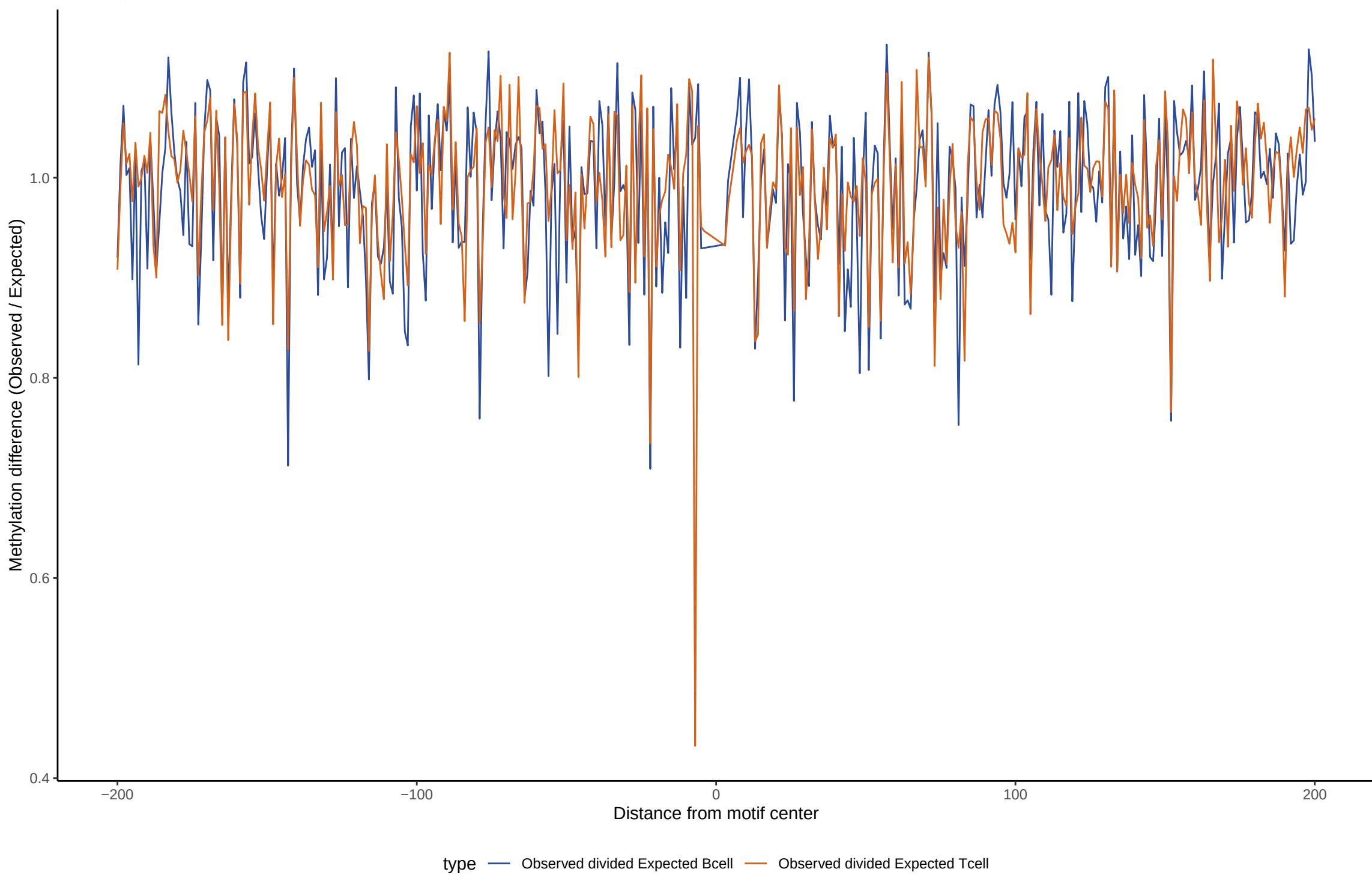
TF footprint difference for MYBL2
