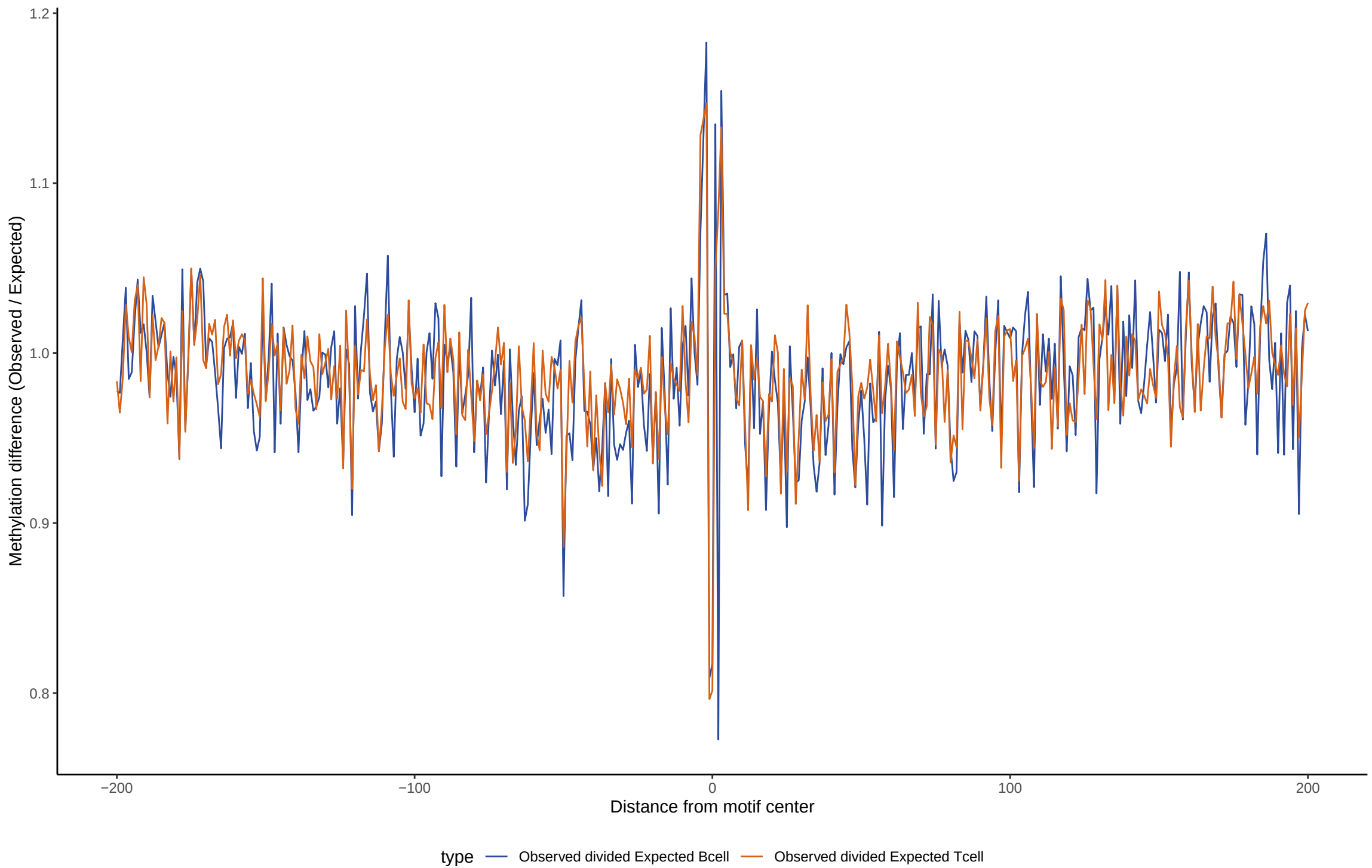
TF footprint difference for MYCN
