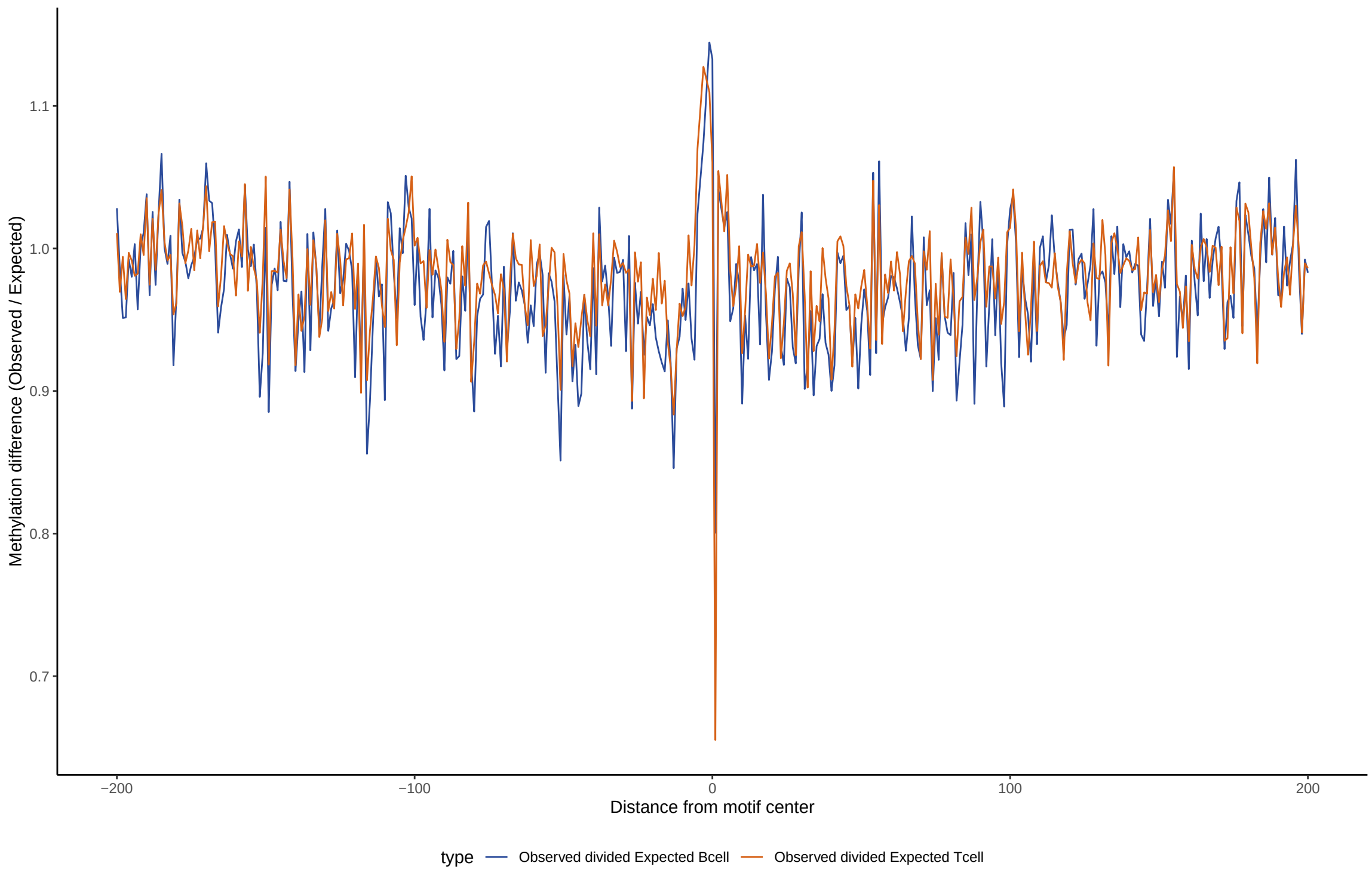
TF footprint difference for MYF6
