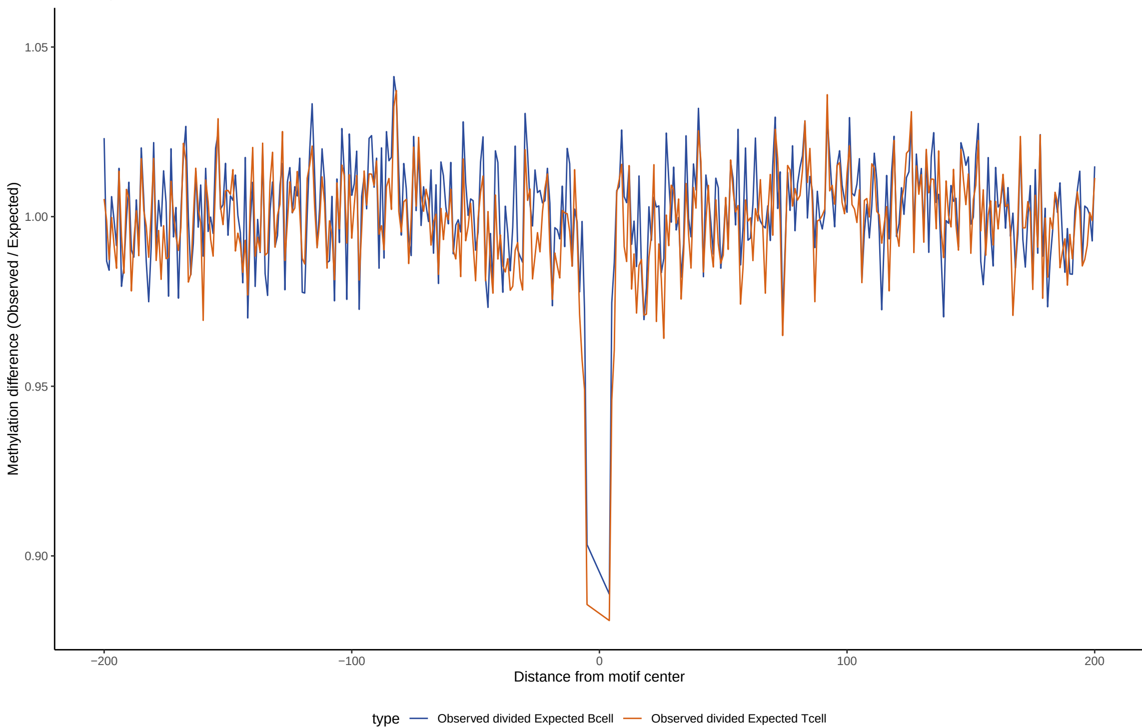
TF footprint difference for NFATC2
