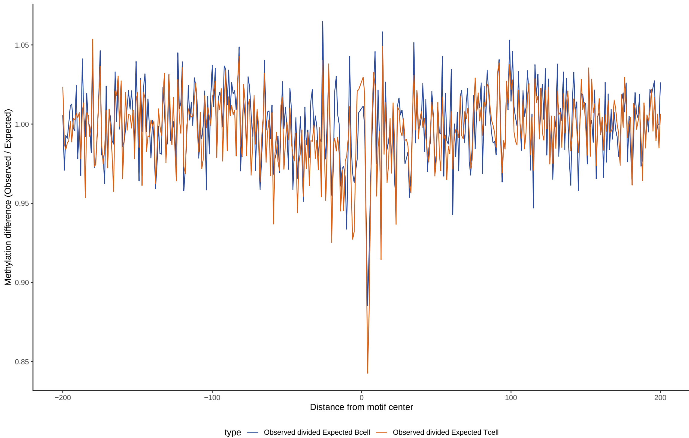
TF footprint difference for NFATC3
