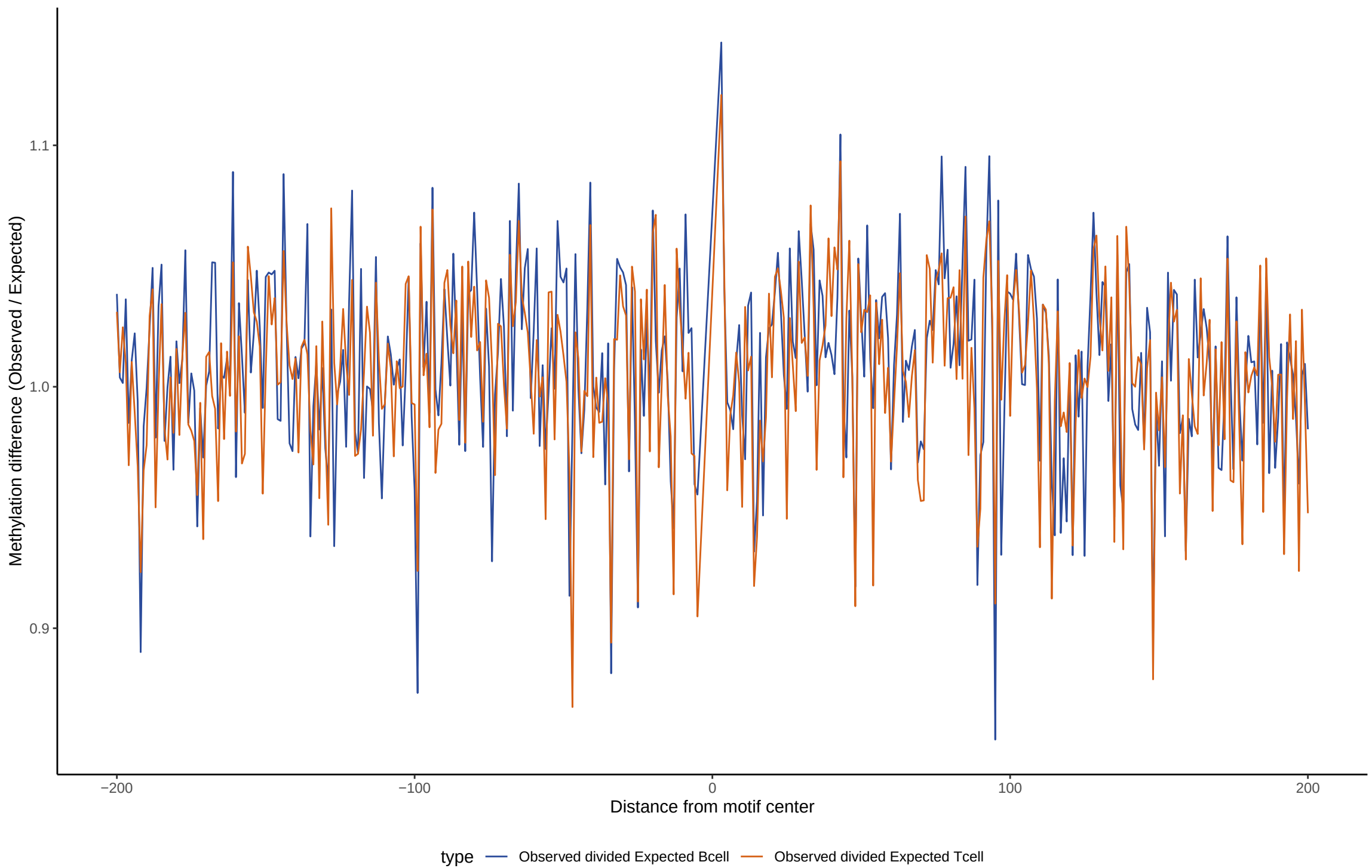
TF footprint difference for NKX6-2
