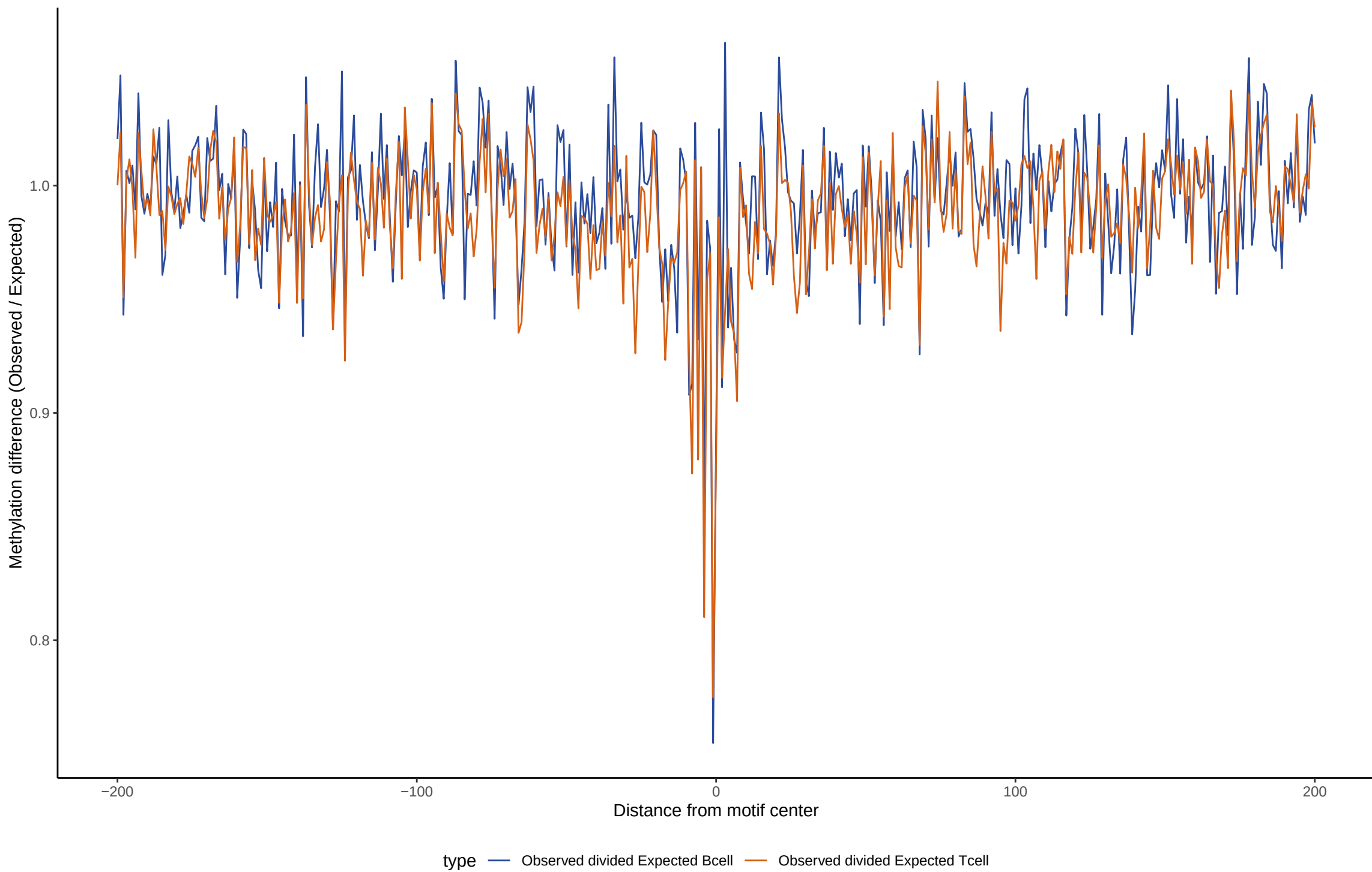
TF footprint difference for NR1H2::RXRA
