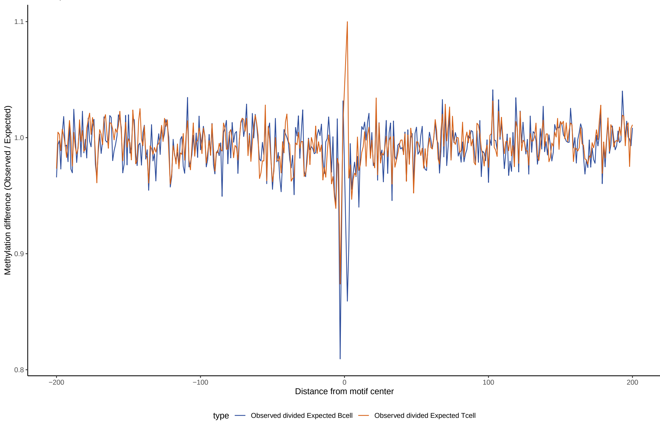
TF footprint difference for NR2C2
