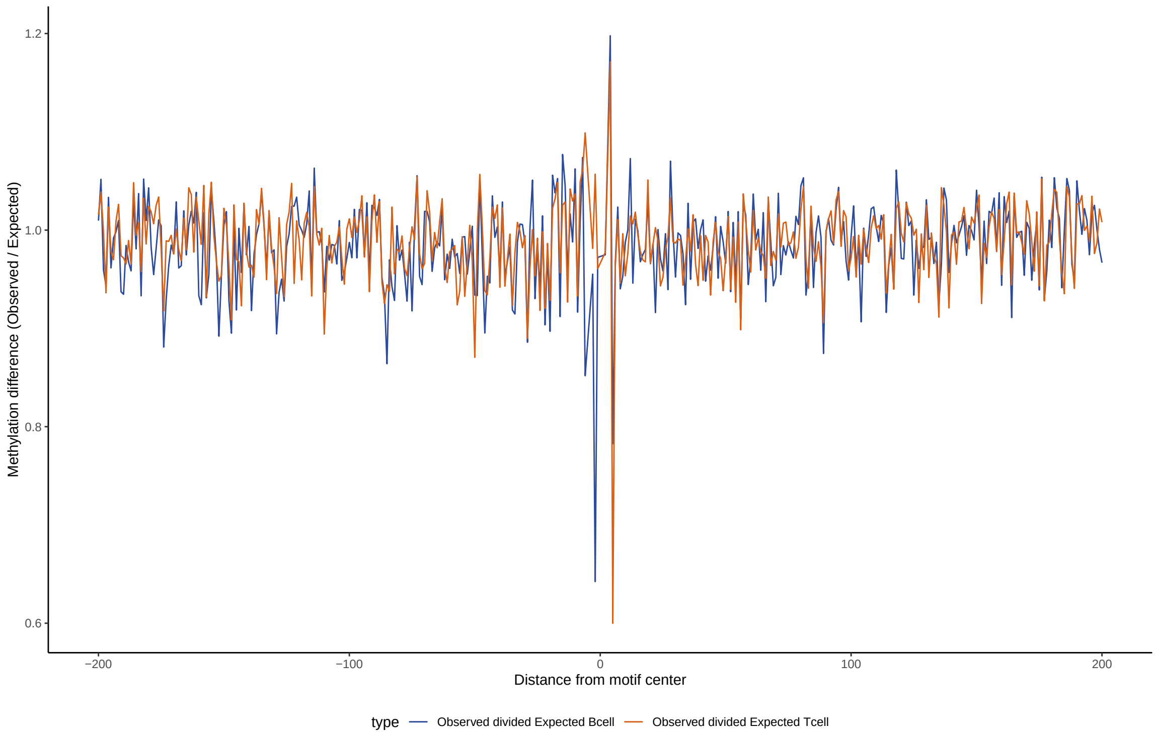
TF footprint difference for NR3C2
