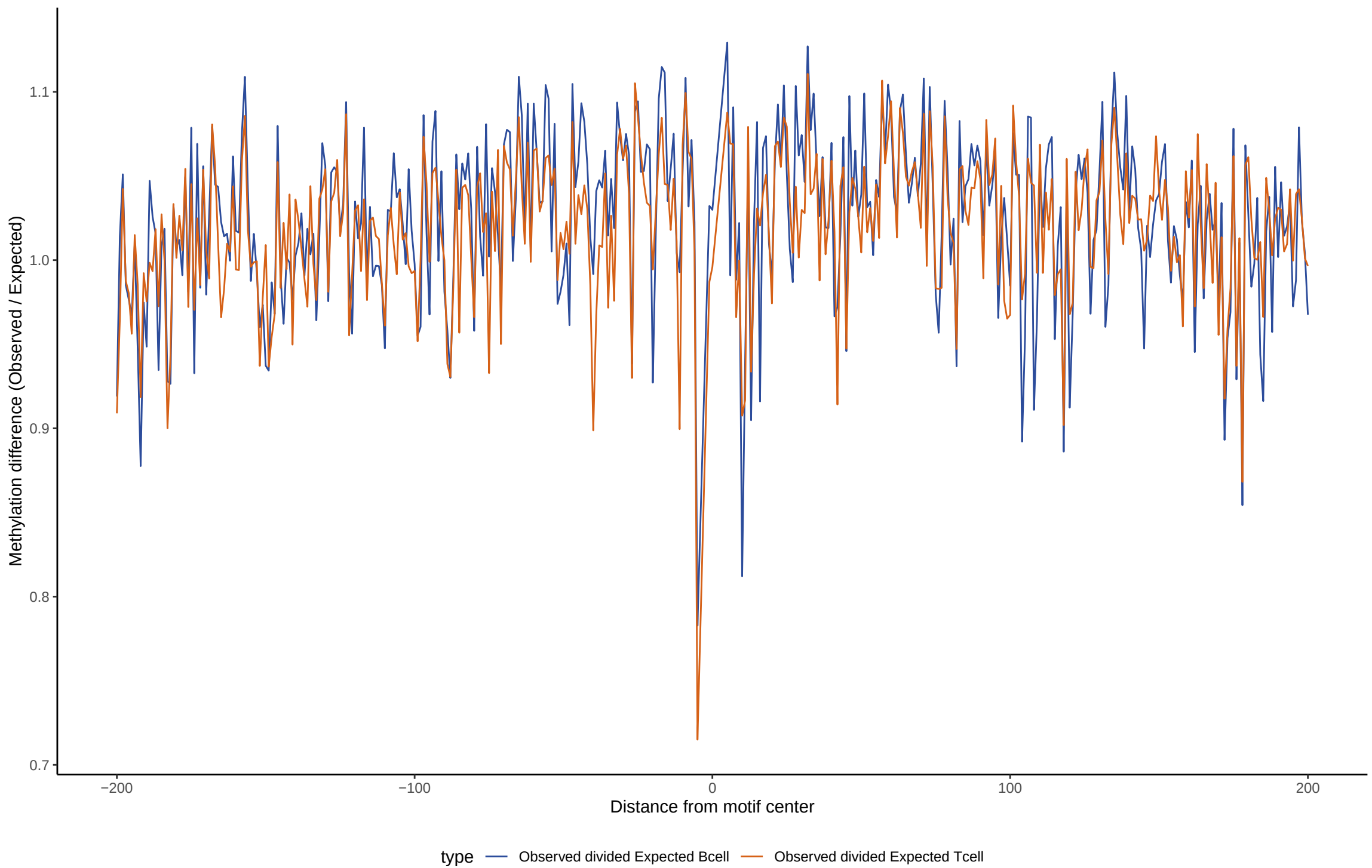
TF footprint difference for PAX7
