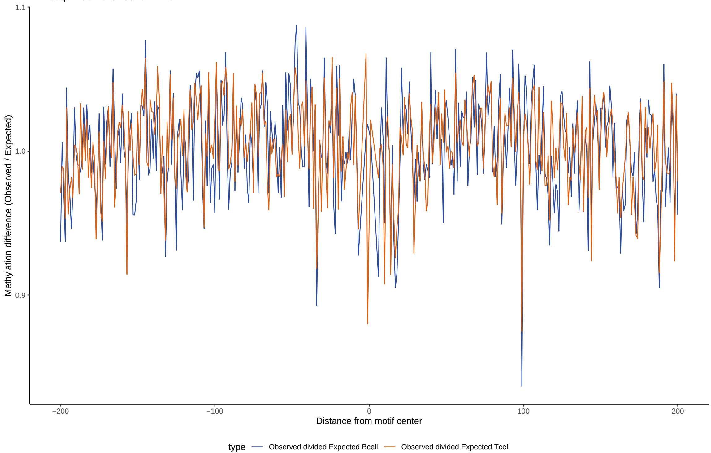
TF footprint difference for PHOX2A
