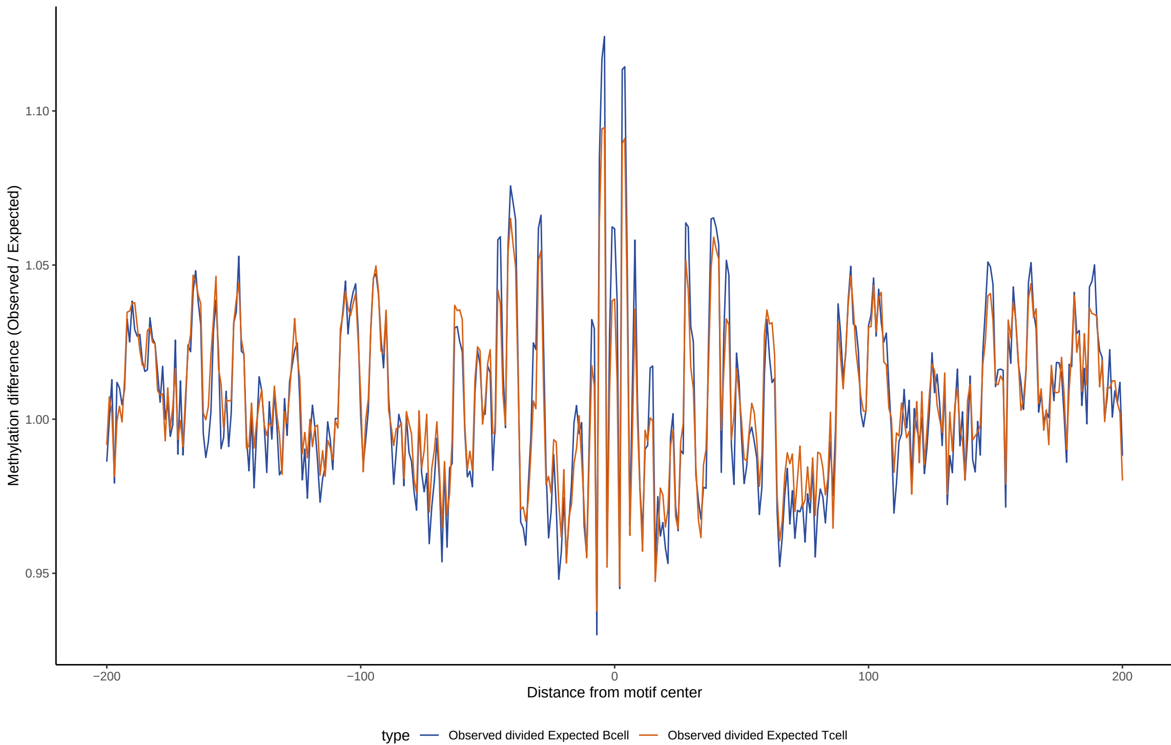
TF footprint difference for PLAG1
