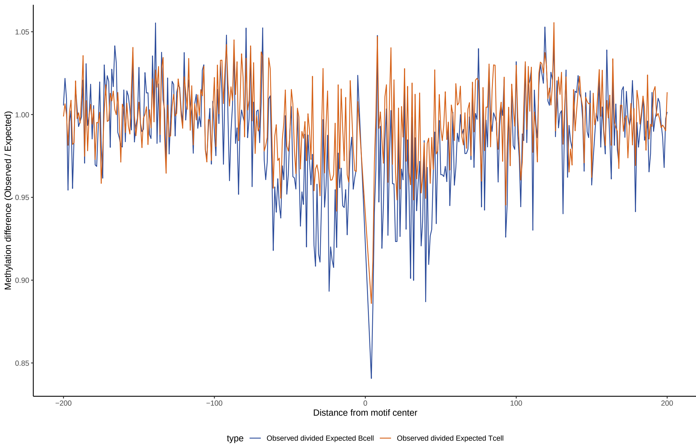
TF footprint difference for POU2F2
