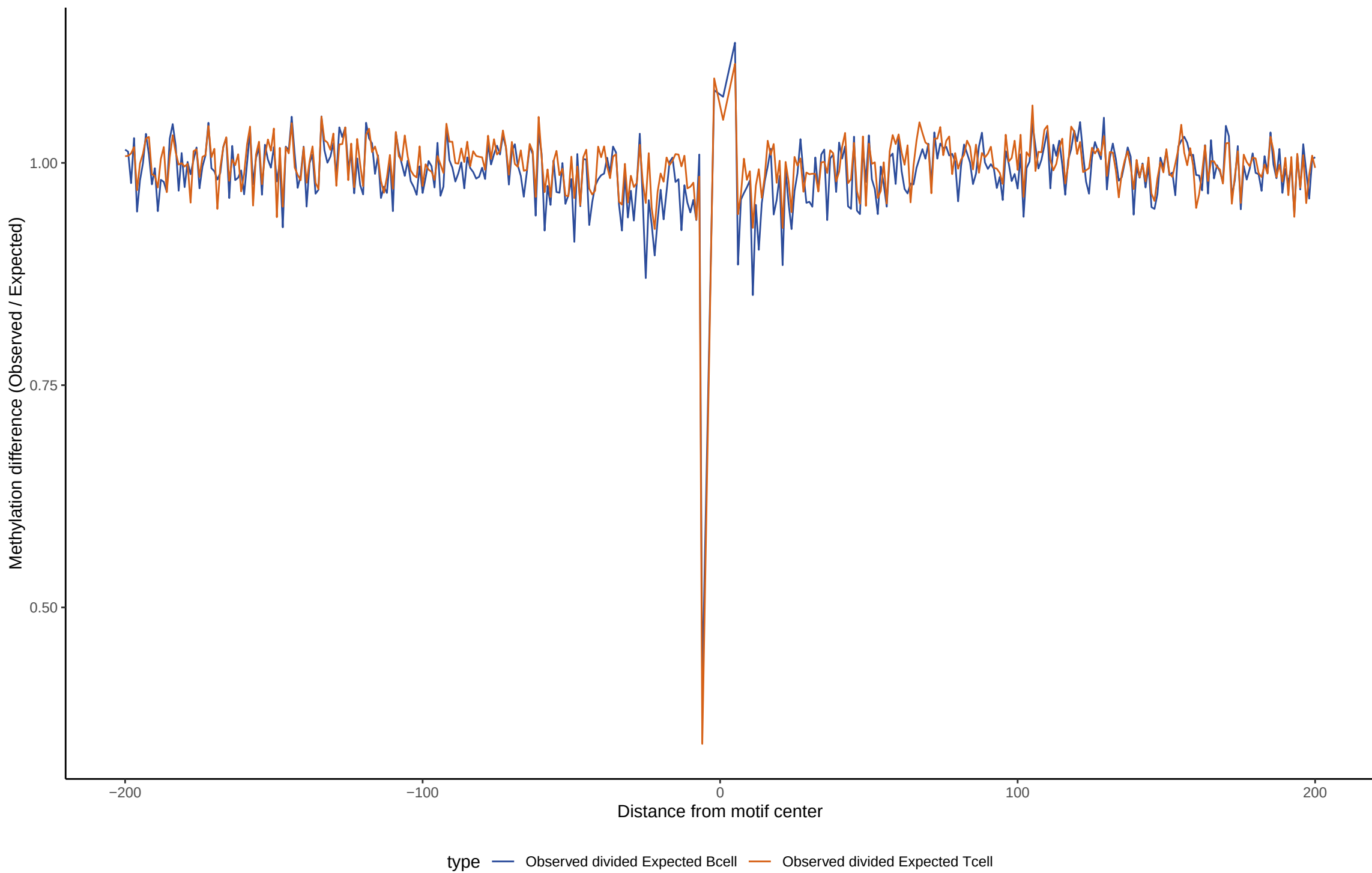
TF footprint difference for POU3F3
