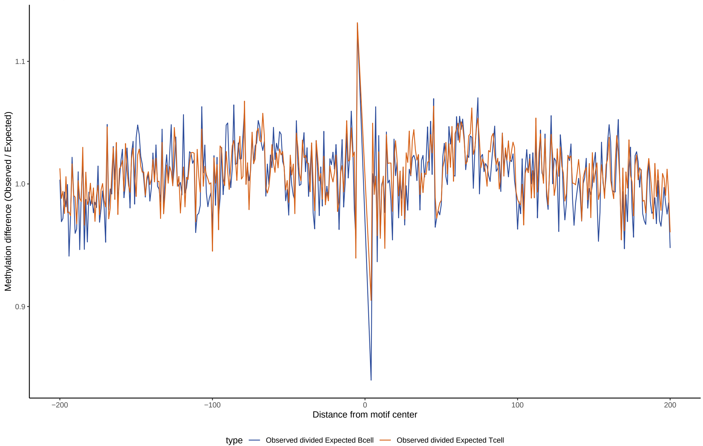
TF footprint difference for POU4F1
