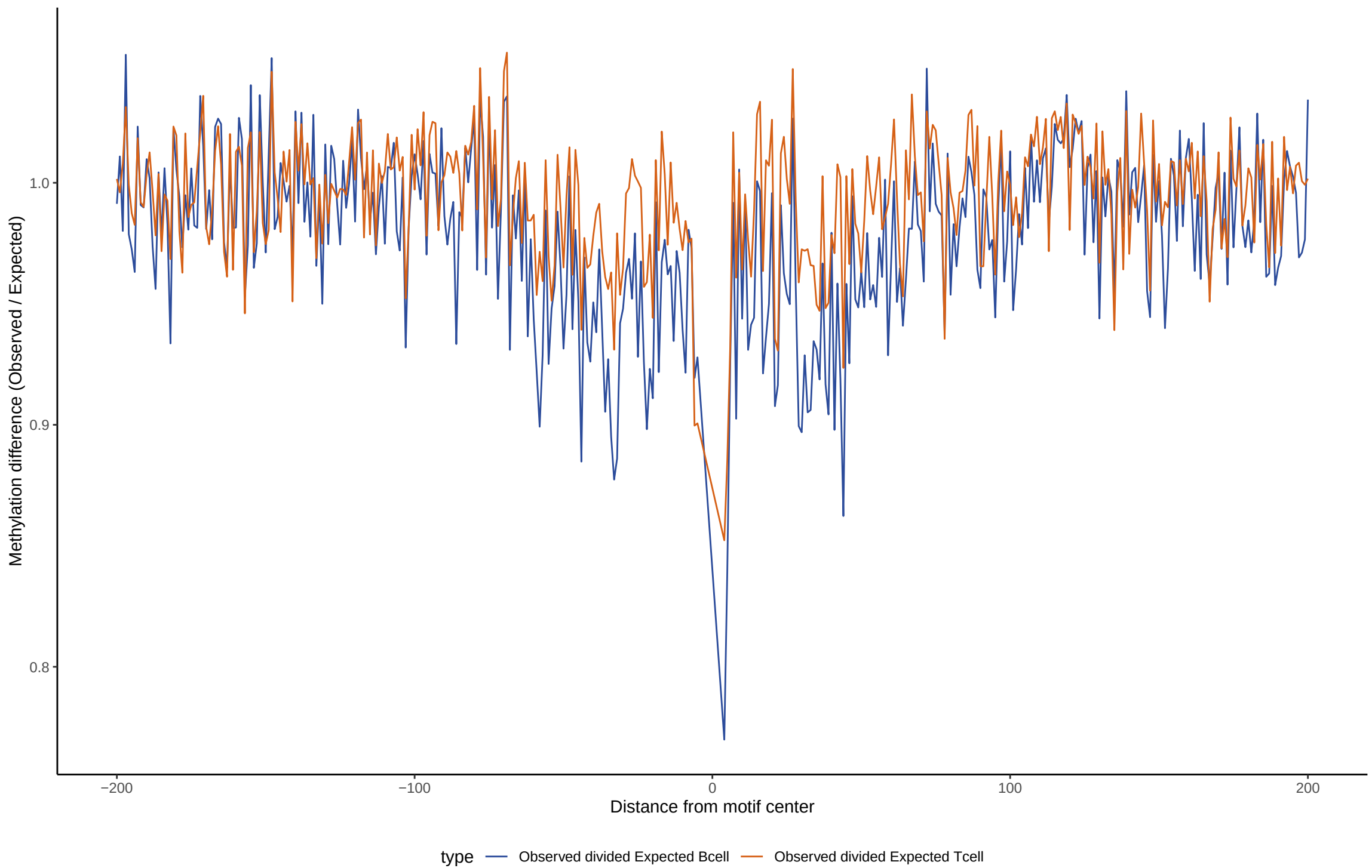
TF footprint difference for POU5F1
