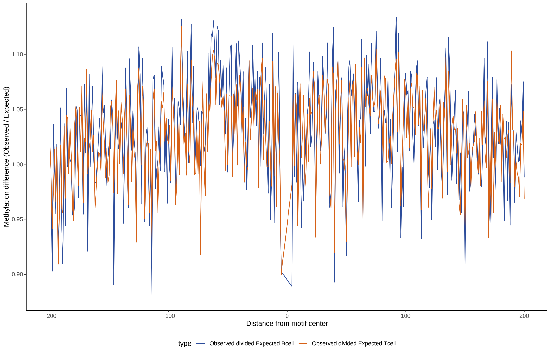
TF footprint difference for POU6F1
