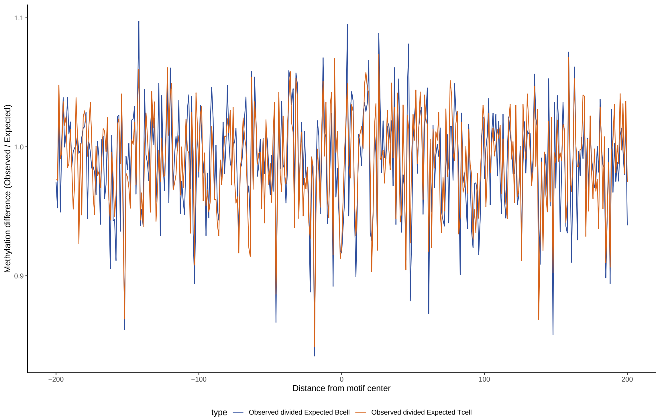
TF footprint difference for PROX1
