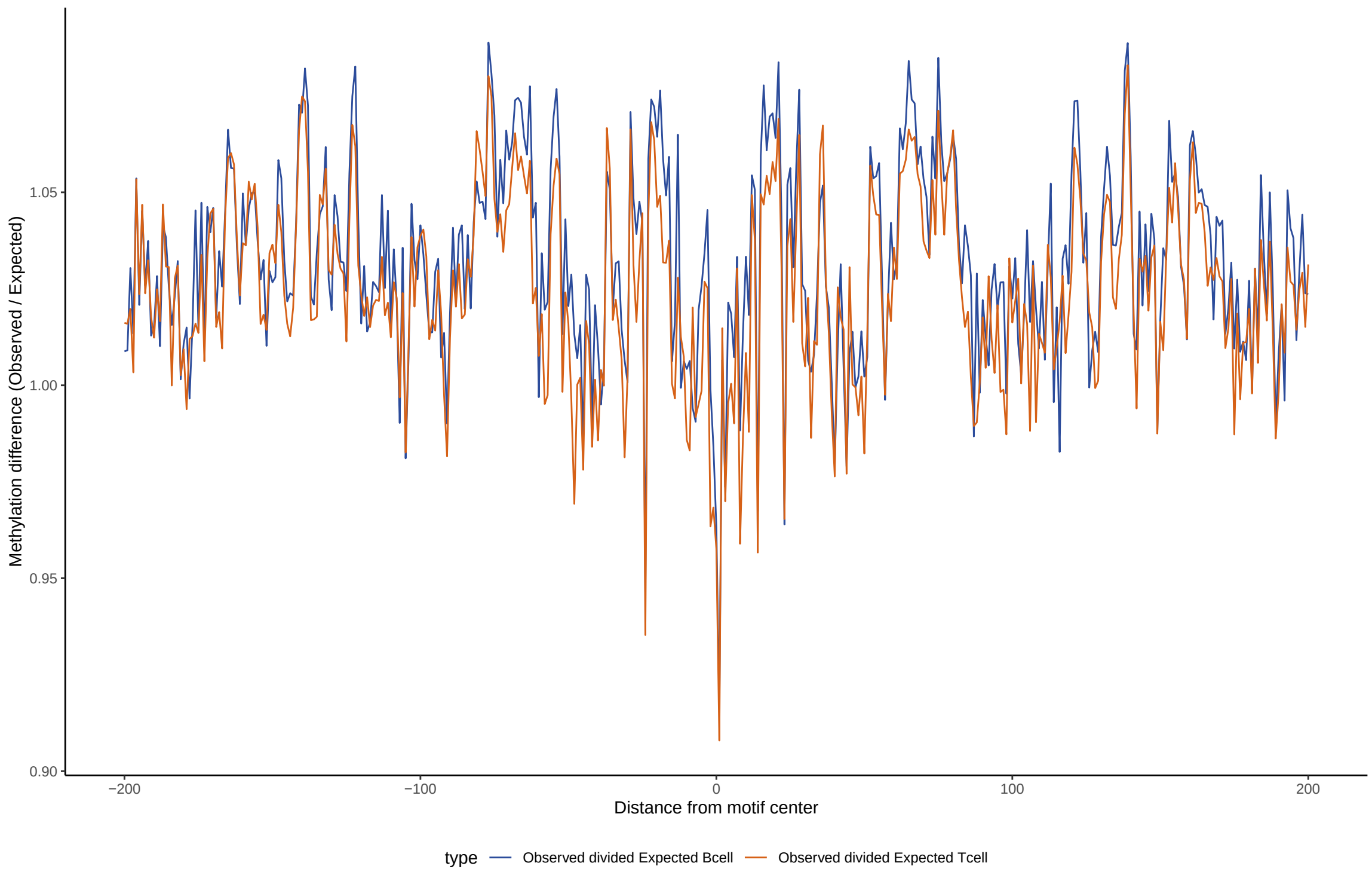
TF footprint difference for RARA
