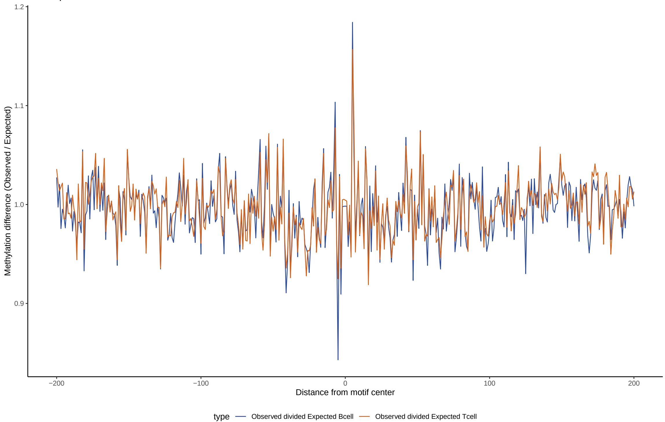
TF footprint difference for RARA::RXRA
