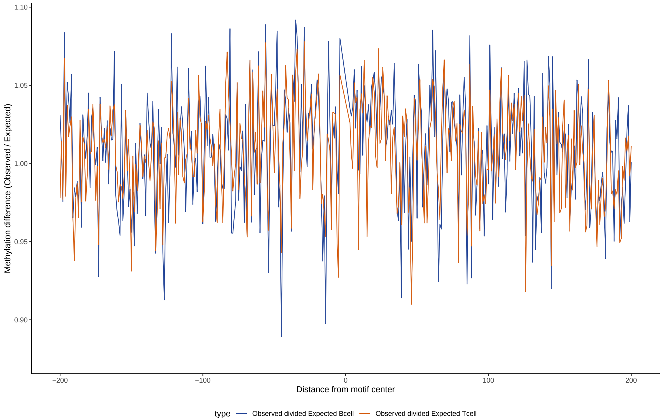
TF footprint difference for RHOXF1
