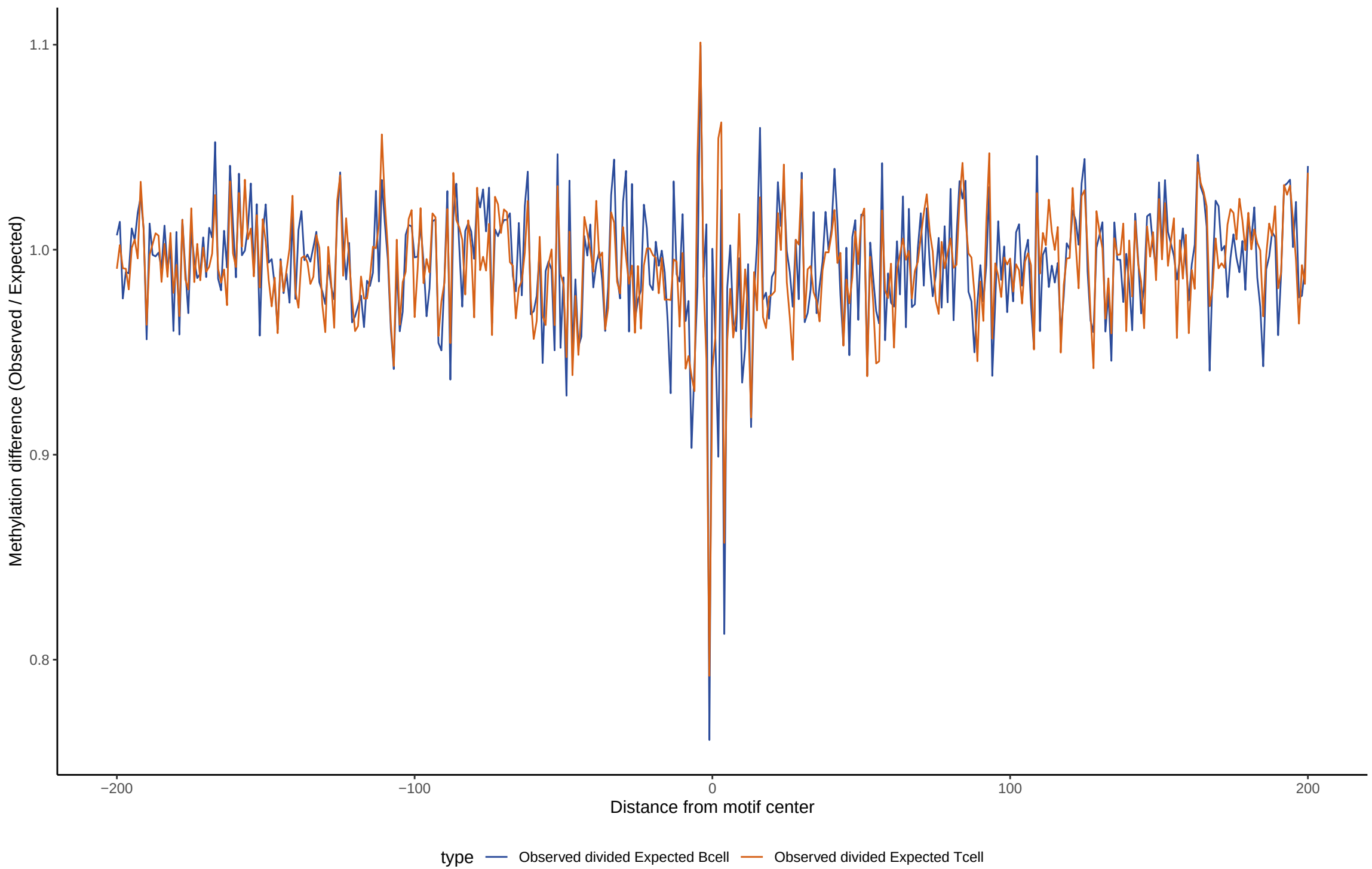
TF footprint difference for RXRG
