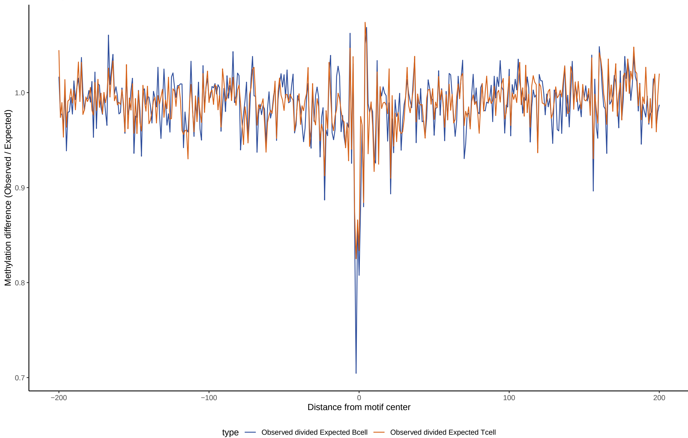
TF footprint difference for SIX2
