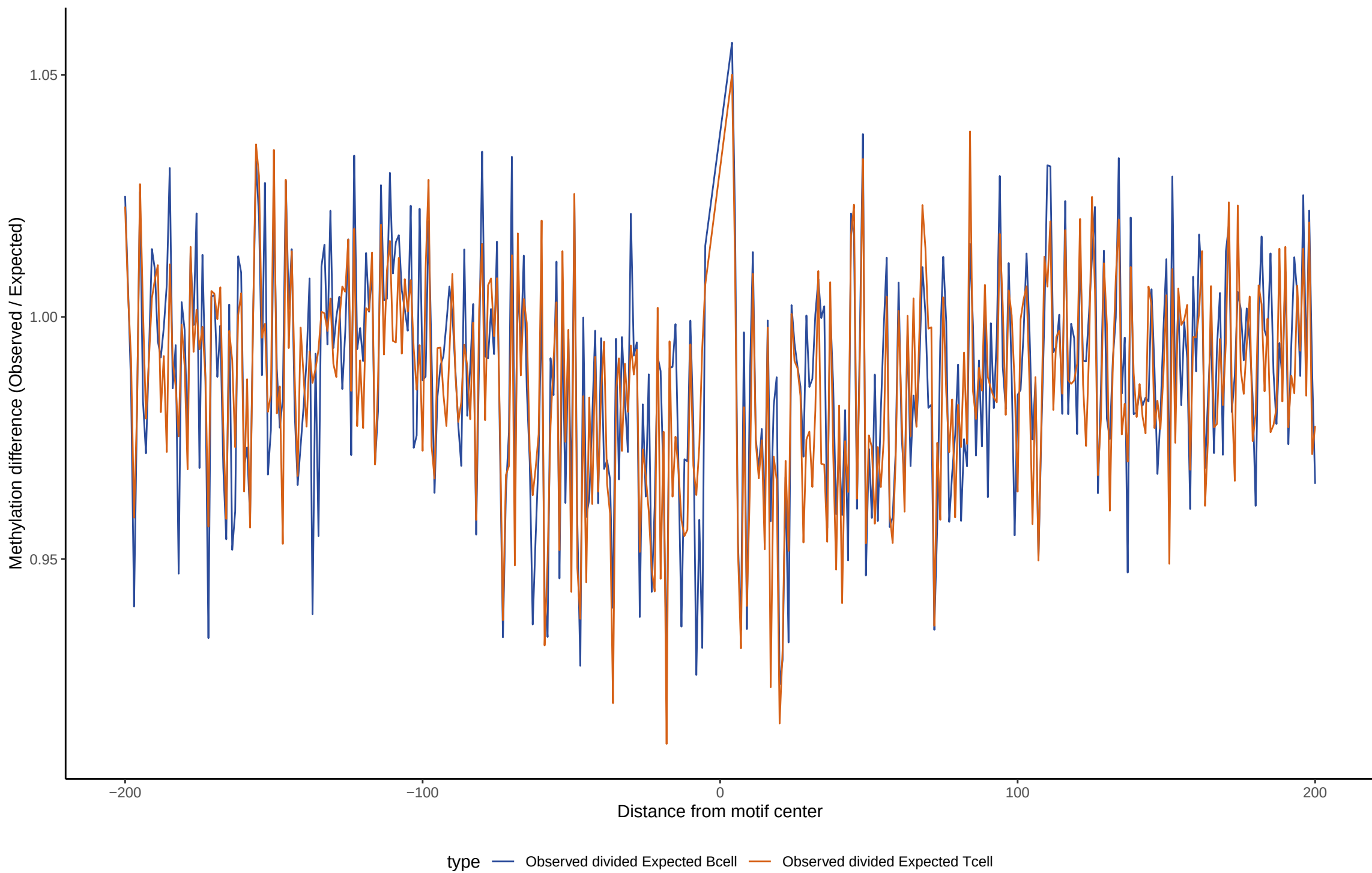
TF footprint difference for SOX10
