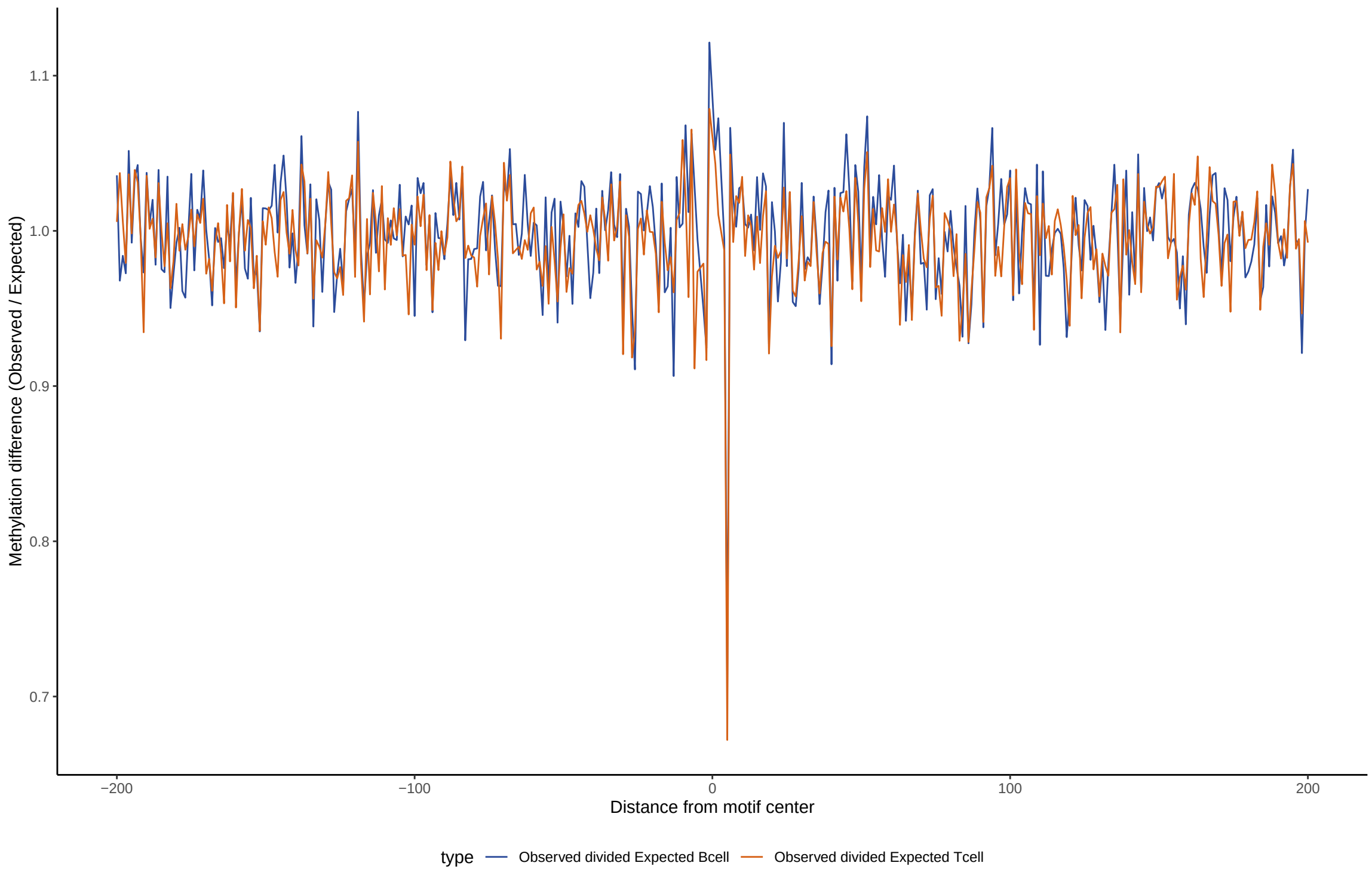
TF footprint difference for SOX21
