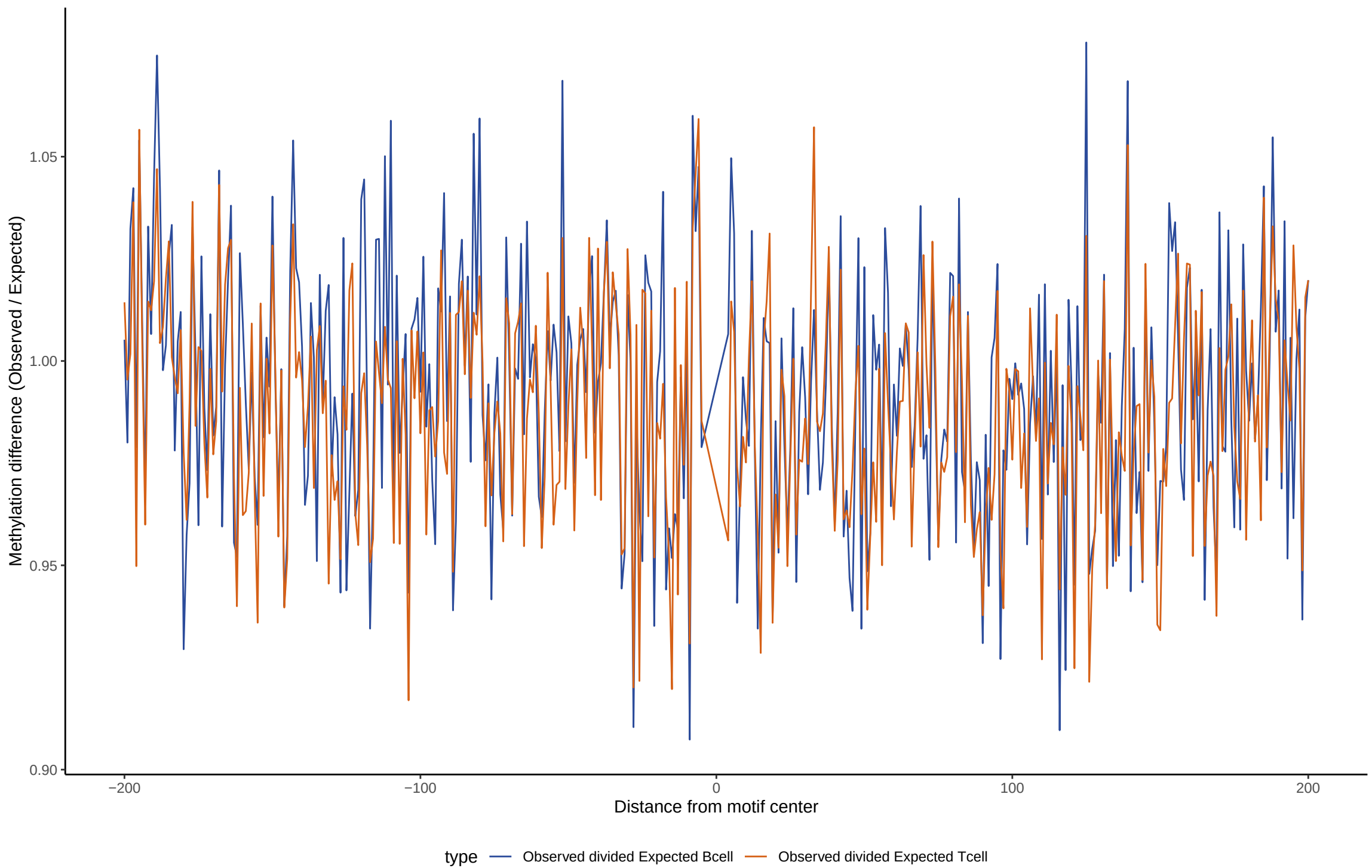
TF footprint difference for SOX9
