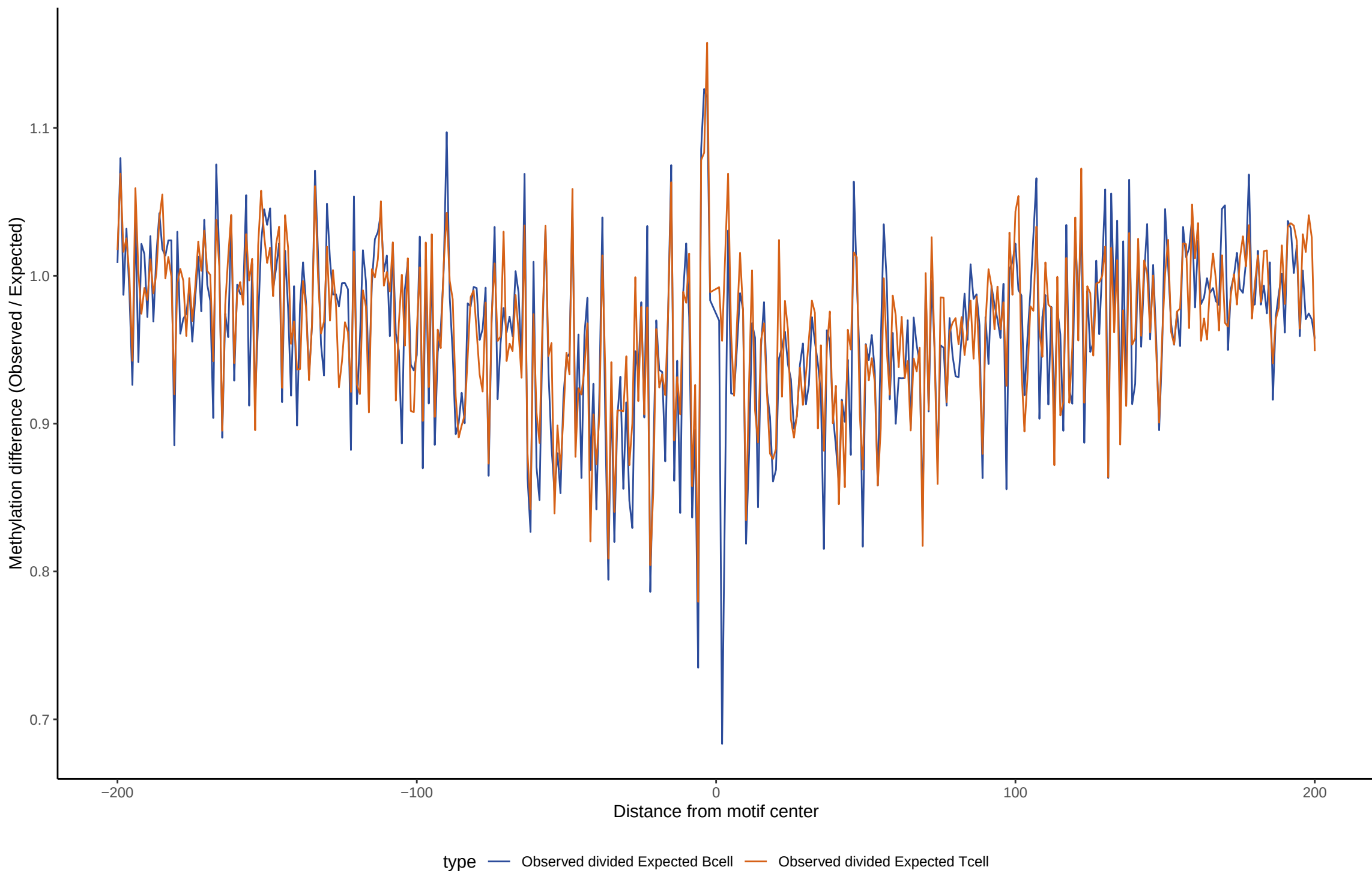
TF footprint difference for SPDEF
