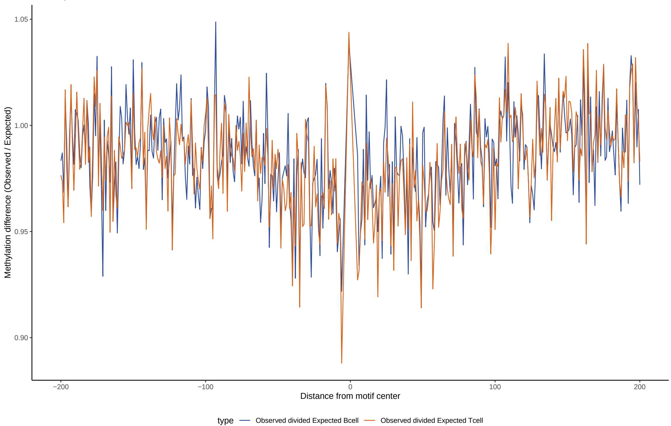
TF footprint difference for STAT3
