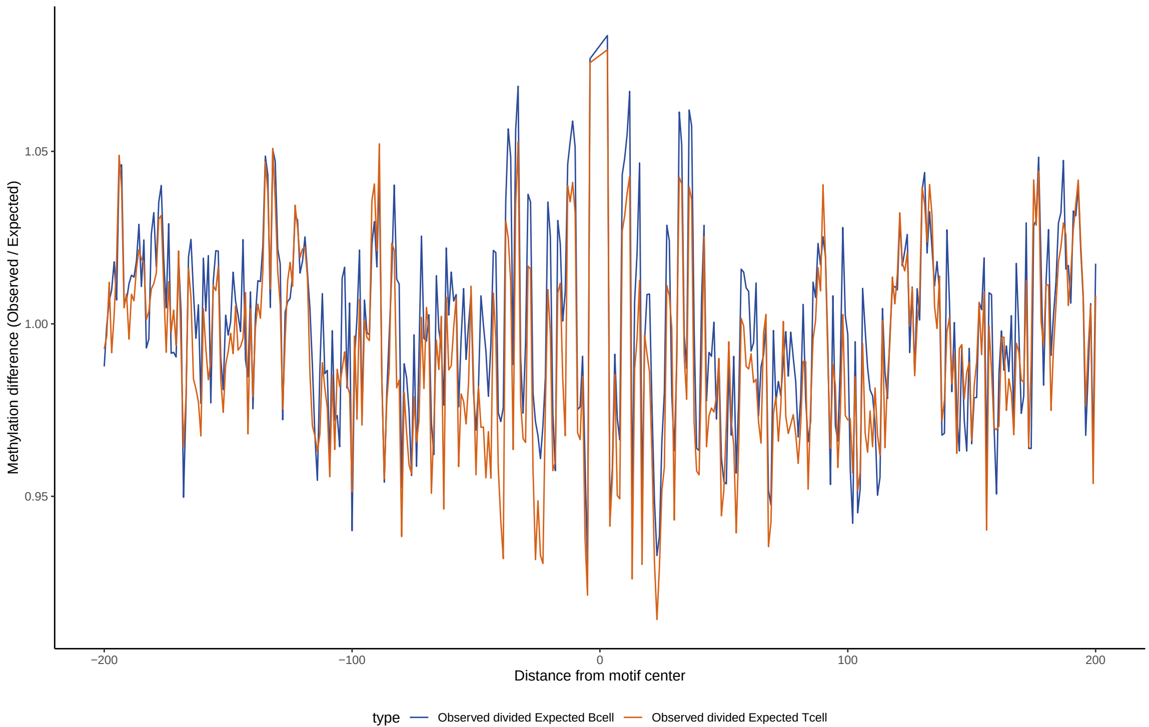
TF footprint difference for TBX5
