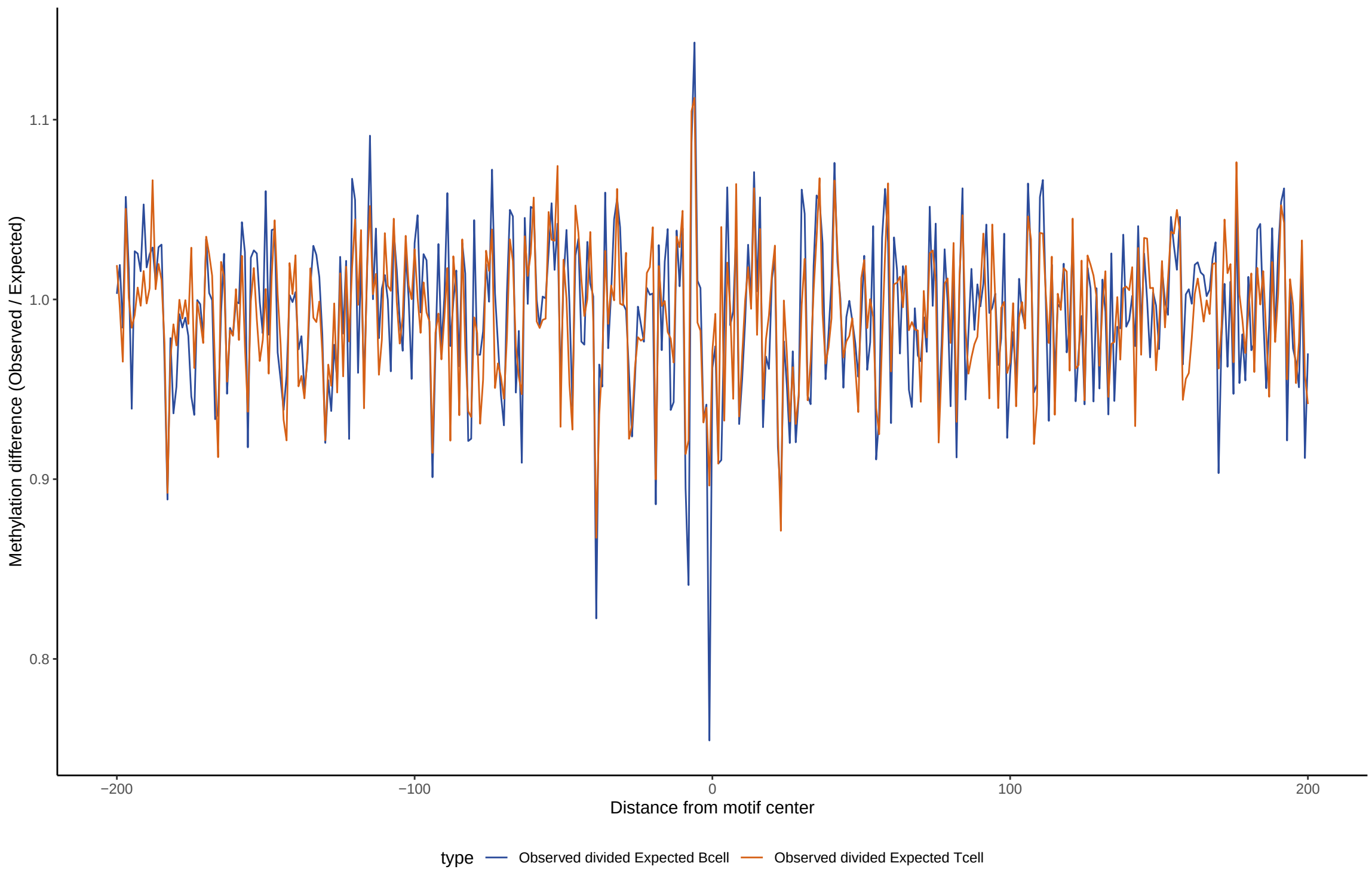
TF footprint difference for TBXT
