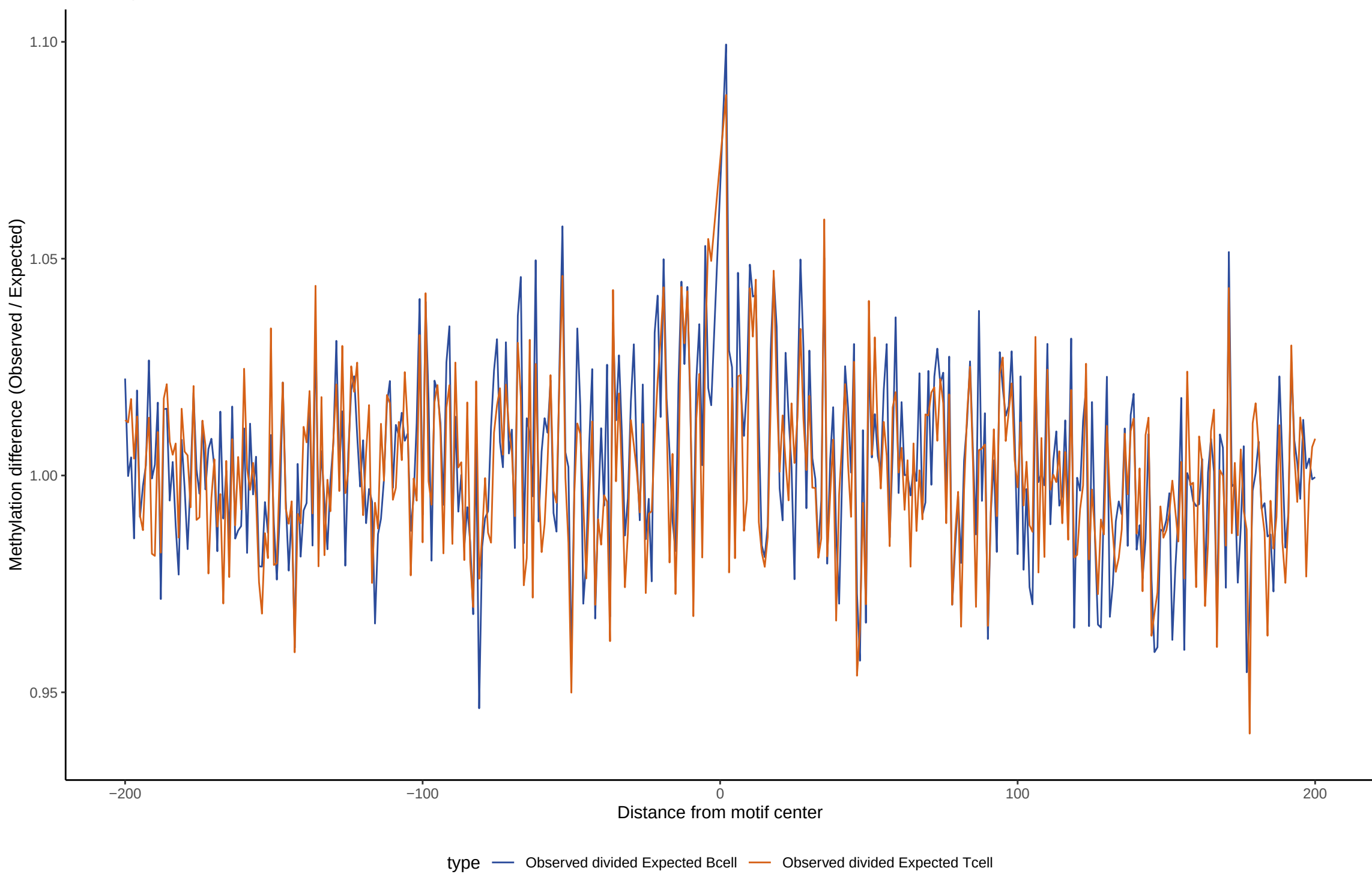
TF footprint difference for TEAD2
